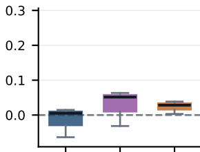
Dist. \Delta
