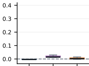
\Delta score
