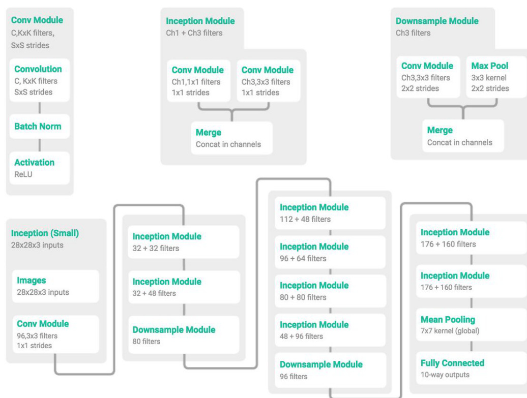
Figure 11.2: The Minicception architecture consists of building blocks including a convolution module, Inception module, and Downsample module. These modules are put together to form the overall architecture.
