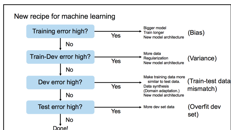
Figure 8.2: Slide 13 of Andrew Ng’s talk [34]. Here Ng proposes four separate data splits when training a deep learning model.
