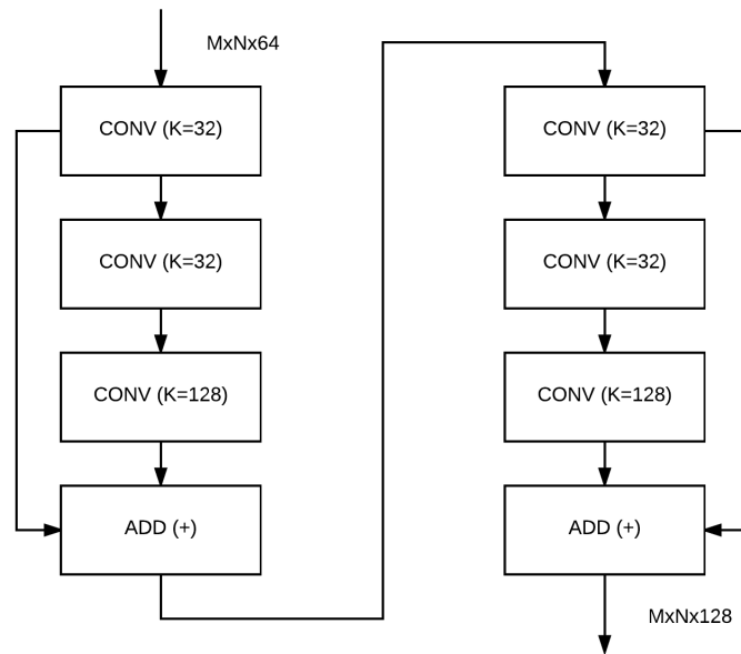
Figure 12.2: An example of two stacked residual modules where one feeds into next. Both modules learn K = 32, 32 , and 128 filters, respectively. Notice how the dimensionality is reduced during the first two CONV layers then increased during the final CONV layer.
