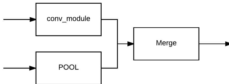
Figure 11.5: The downsample_module is responsible for reducing the spatial dimensions of our input volume. The first branch learns a set of filters with 2 \times 2 stride to reduce the output volume. The second branch also reduces the spatial dimensions, this time by applying max pooling. The output of the downsample_module is concatenated along the channel dimension.
