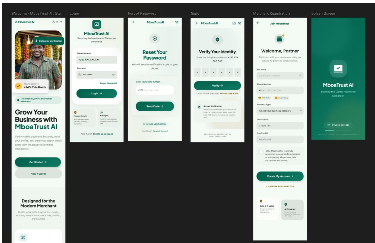
Figure A1. Entry, onboarding, registration, and access screens.
