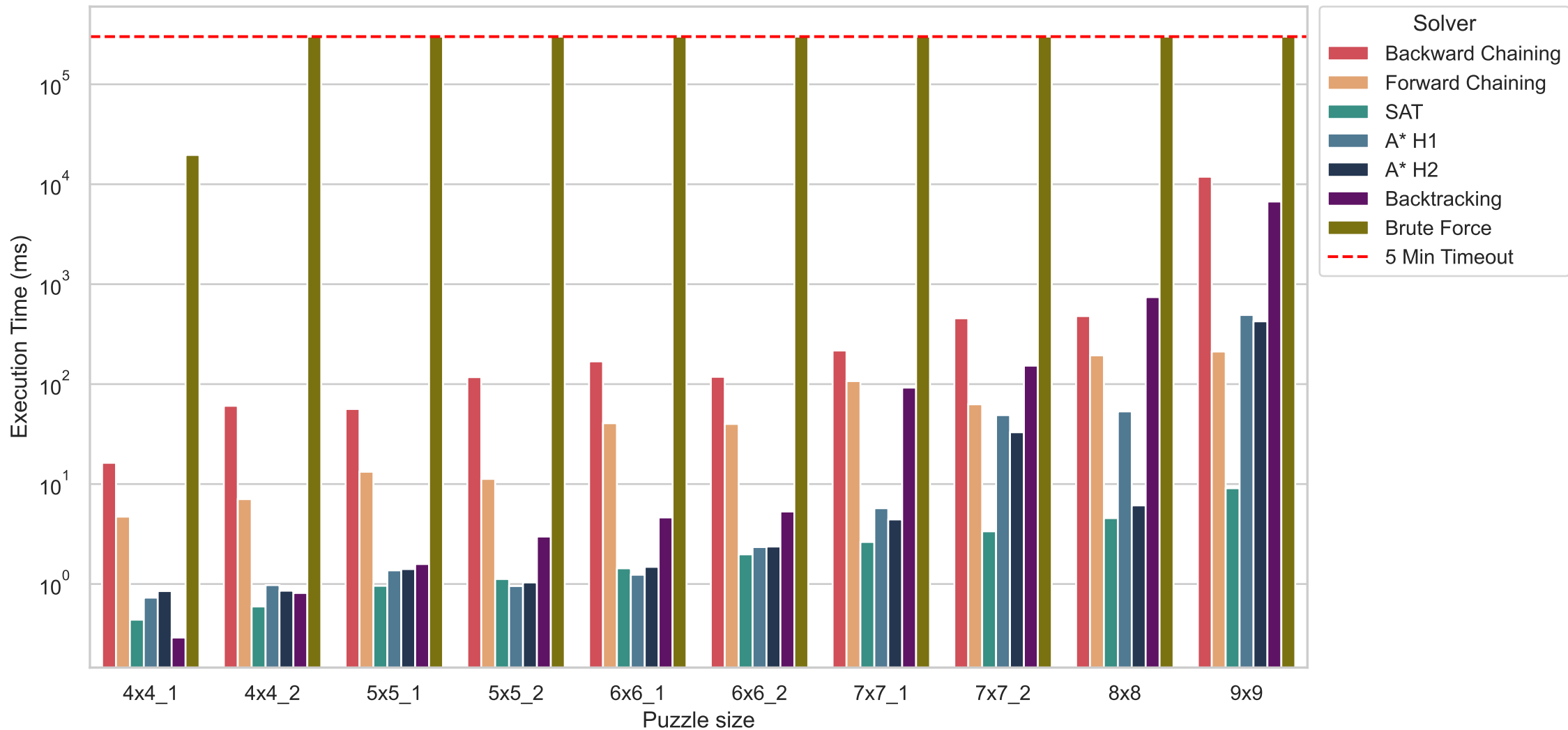
Solver Execution Time
