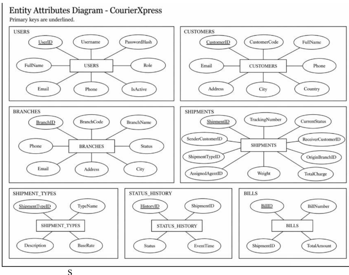
Figure 4. Entity Attributes
