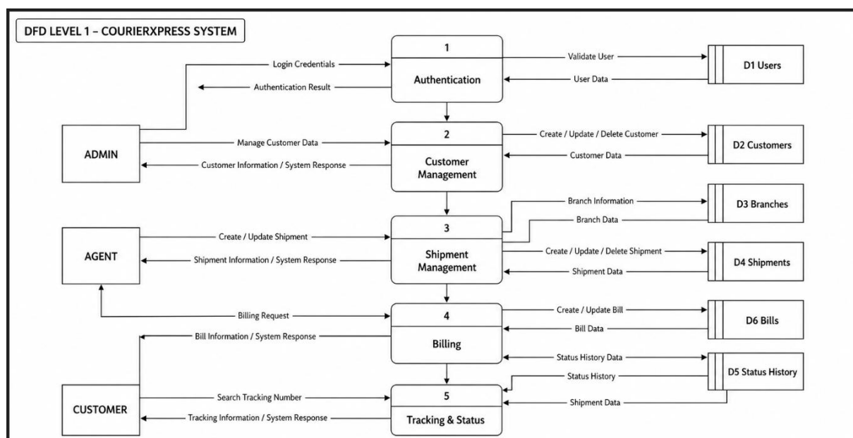
Figure 2. DFD Level 1
