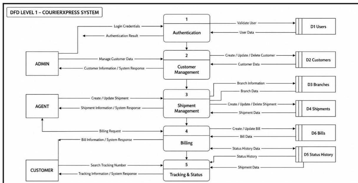
Figure 2. DFD Level 1
