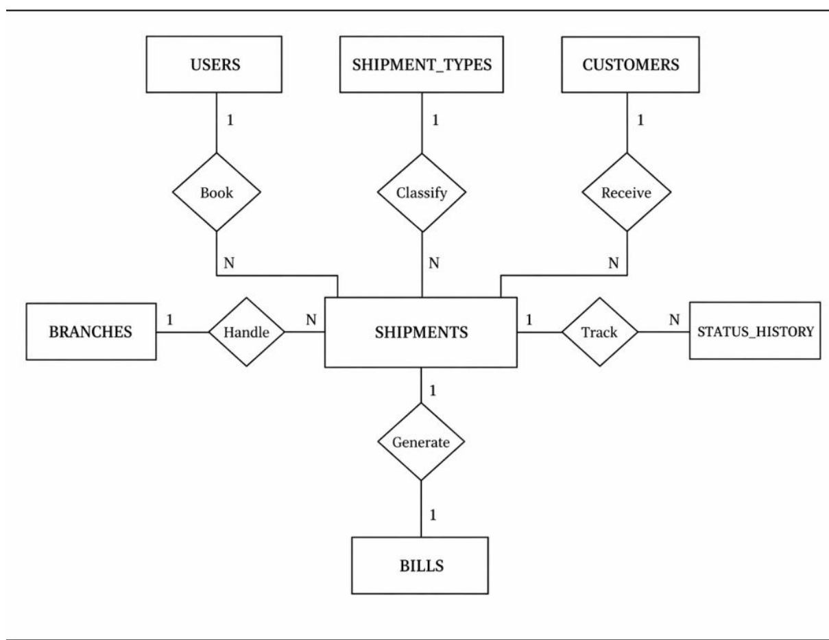
Figure 3. Conceptual ERD
