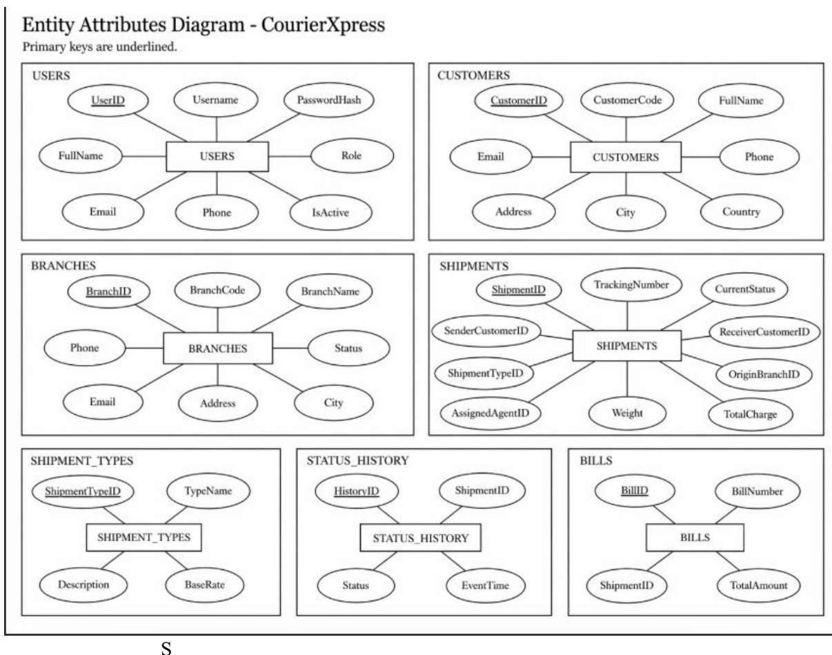
Figure 4. Entity Attributes
