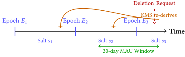
Figure 2: Epoch timeline showing salt rotation and retroactive deletion (schematic; not to scale —each epoch spans 365 days while the query window spans 30). When a deletion request arrives, the KMS re-derives historical hashes using retained salt seeds ( s_1, s_2 ) to generate tombstones for all affected days within the MAU window.
