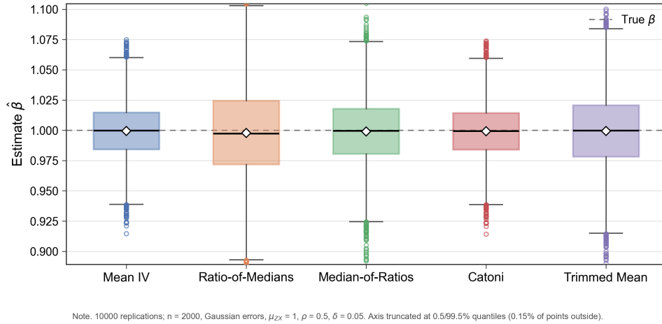
Figure 1: Boxplot showing the cost of robustness under Gaussian errors
