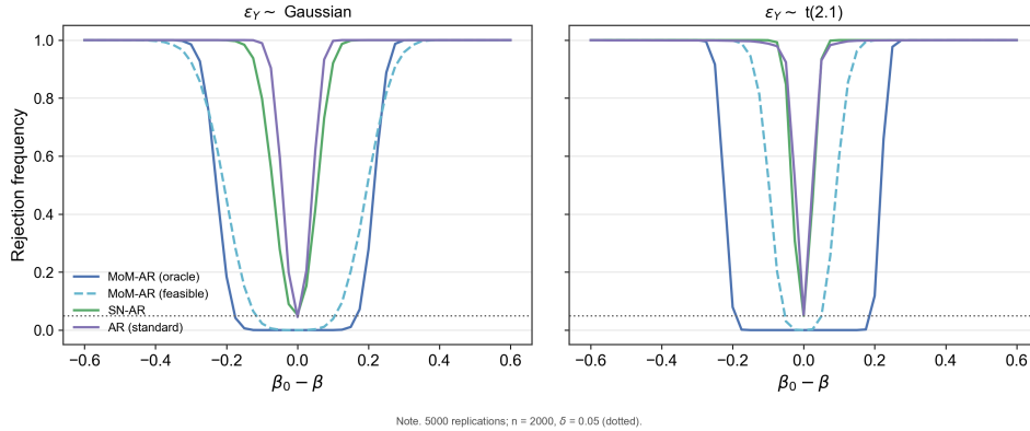
Figure 7: Power curves of all tests
