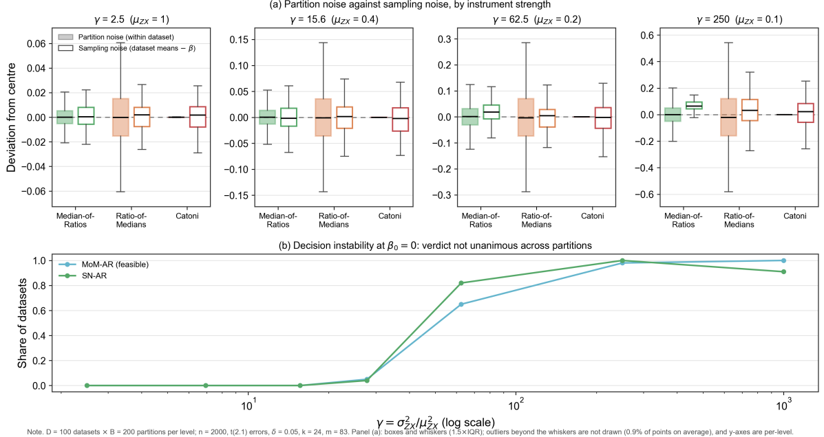
Figure 8: Partition noise against sampling noise, and the share of datasets whose test verdict at \beta_0 = 0 depends on the partition, against instrument strength \gamma = \sigma_{ZX}^2 / \mu_{ZX}^2
