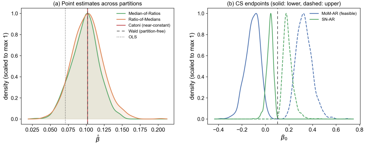
Figure 10: Partition sensitivity on the Angrist and Krueger (1991) extract over B = 1,000 random partitions. Panel (a): kernel density estimates of the point estimates, each scaled to unit maximum, with the partition-free Wald and OLS values marked. Panel (b): densities of the outer endpoints of the 95% confidence sets (solid: lower, dashed: upper).
