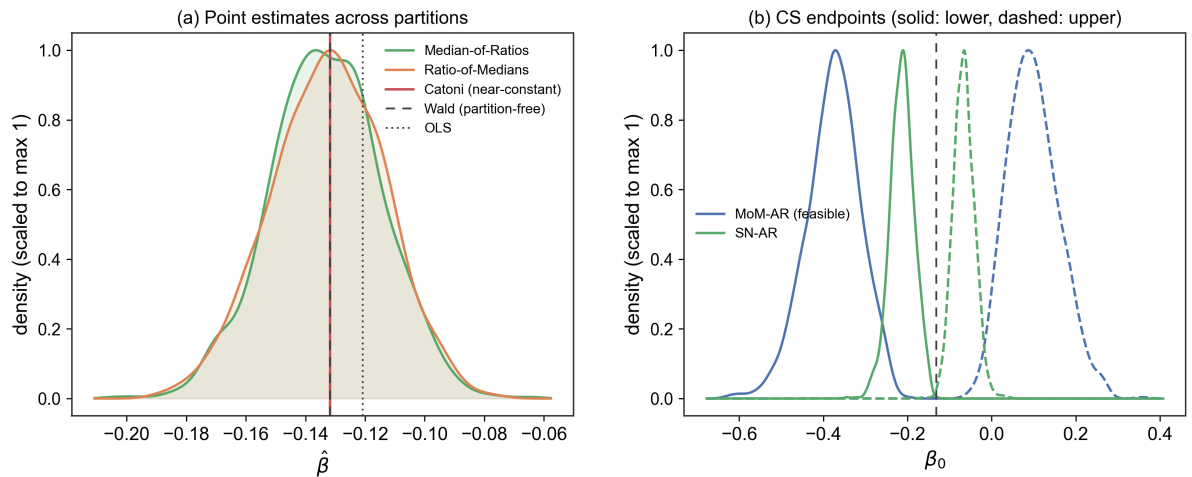
Figure 11: Partition sensitivity for Worked for pay, Angrist and Evans (1998) 1980 all-women sample, B = 1,000 random partitions. Panels as in Figure 10.
