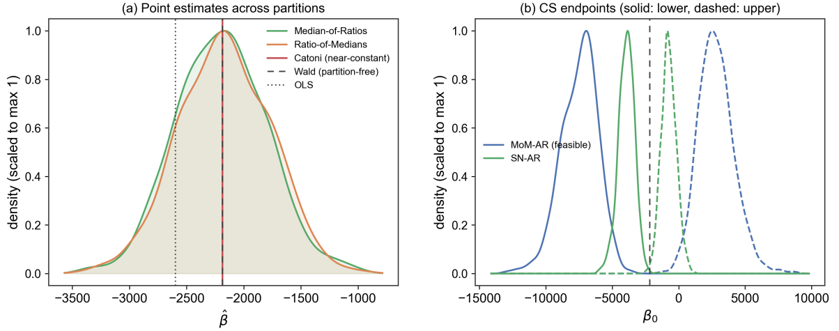
Figure 12: Partition sensitivity for Labour income, Angrist and Evans (1998) 1980 all-women sample, B = 1,000 random partitions. Panels as in Figure 10.
