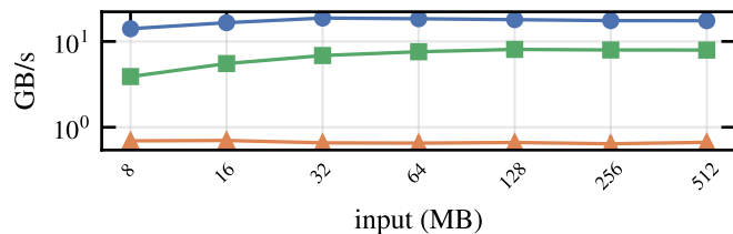
C-like
