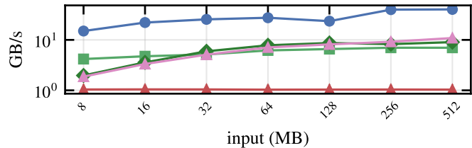
TOML
