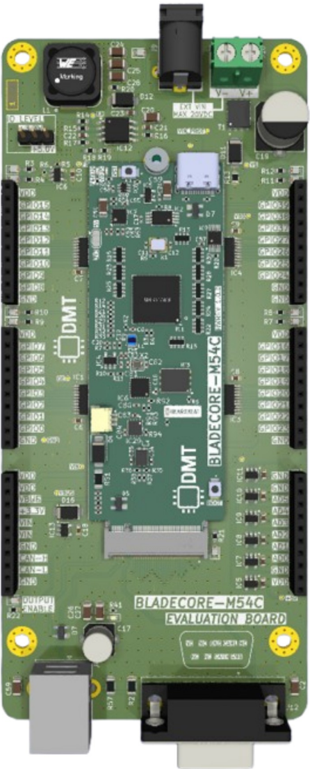
TOP VIEW
