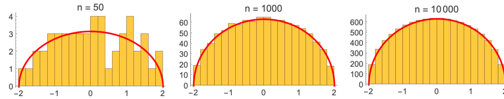
Fig. 1: Simulation of Wigner's Semicircle Law
