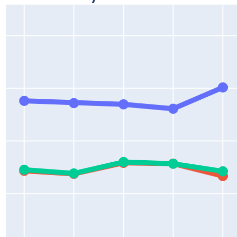
Entity Detection
