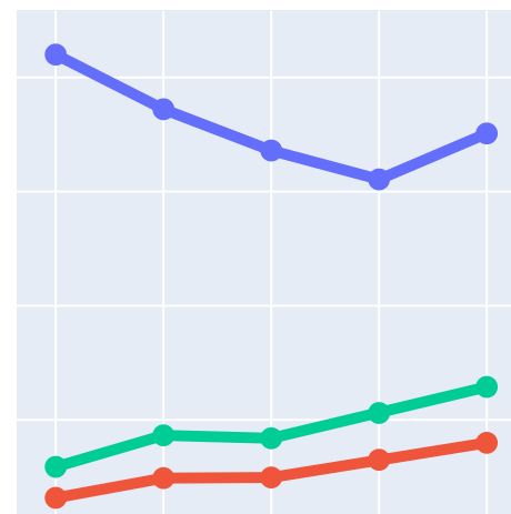
Event Detection
