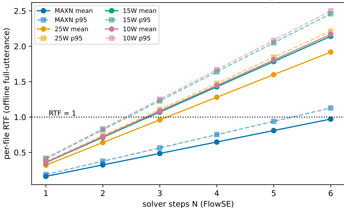
Fig 6.1 Solver-step budget on Orin NX (jetson_clocks on)
