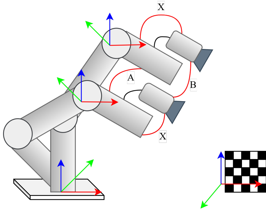
Fig. S.1: Formulating the AX=XB problem.
