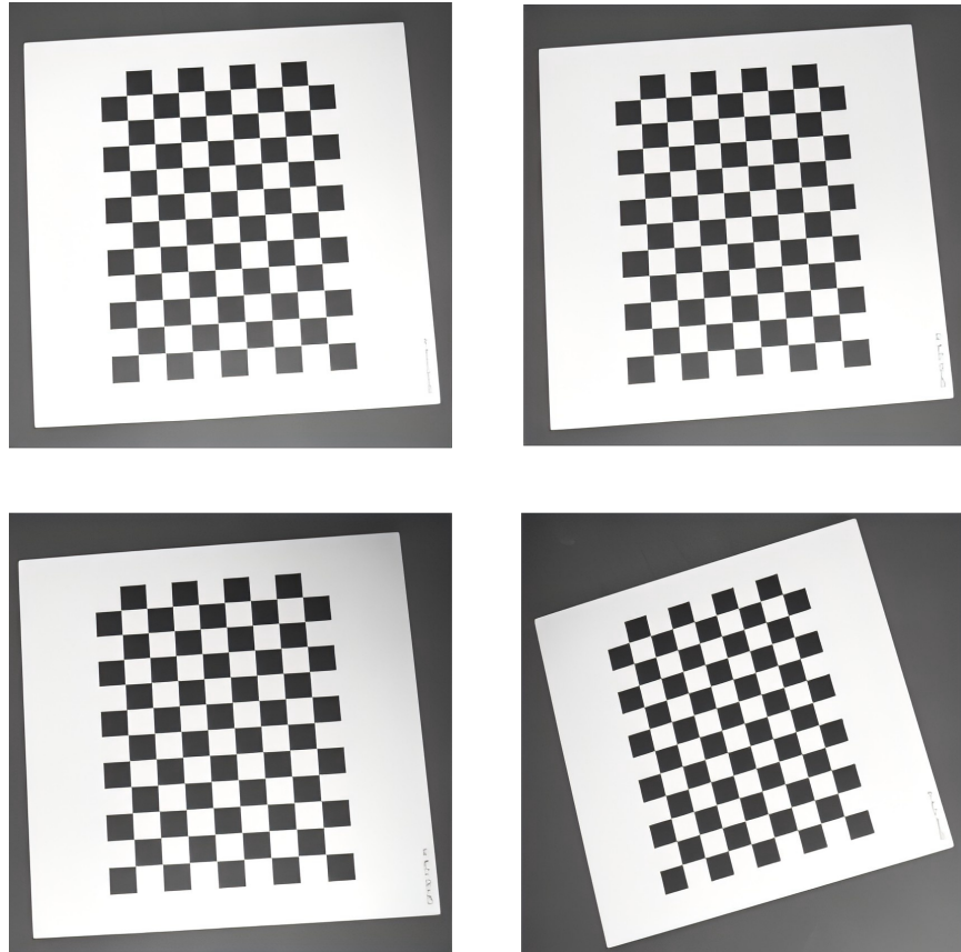
Fig. S.2: Images of the calibration board captured from different poses.
