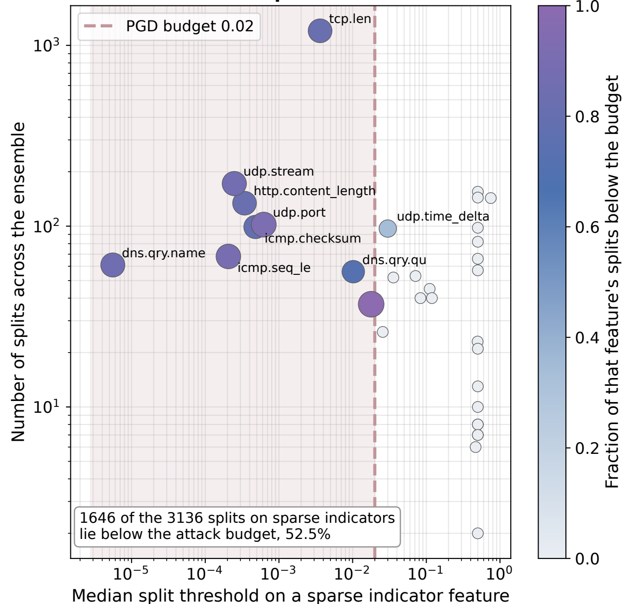
Where the forest places its thresholds
