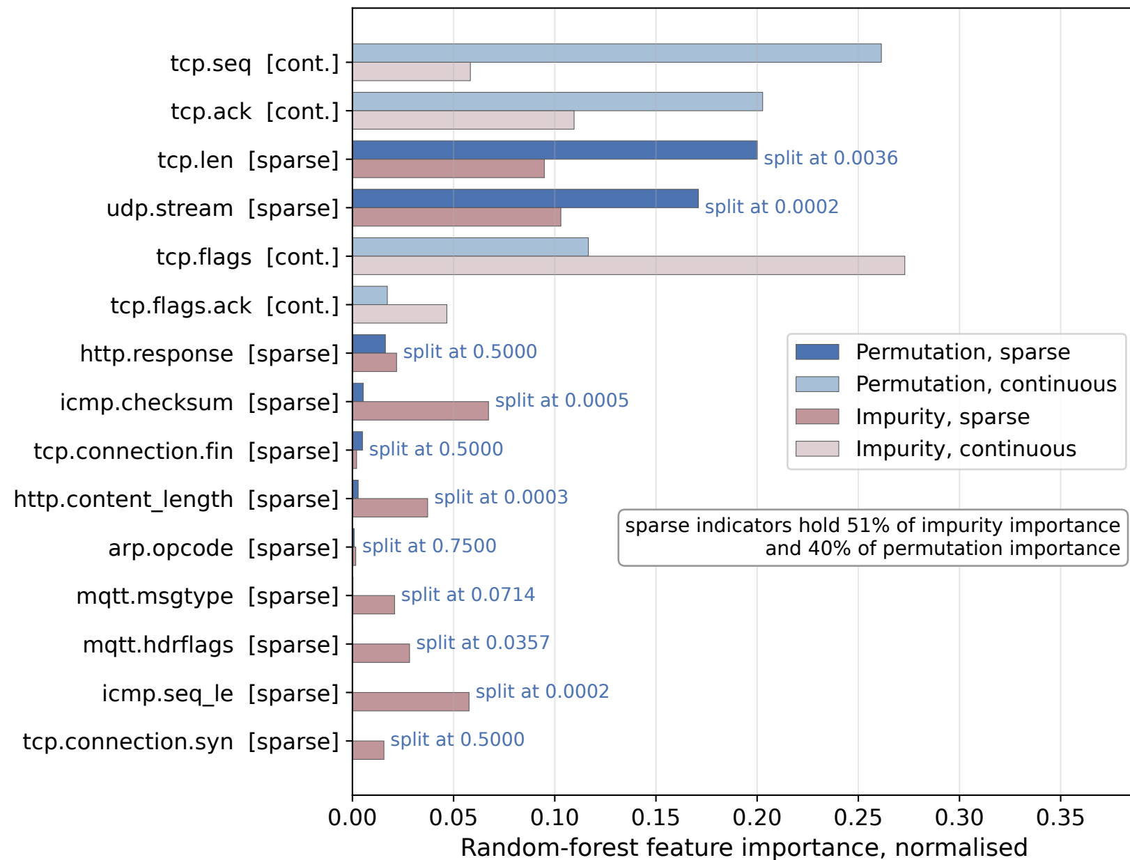
What the forest relies on
