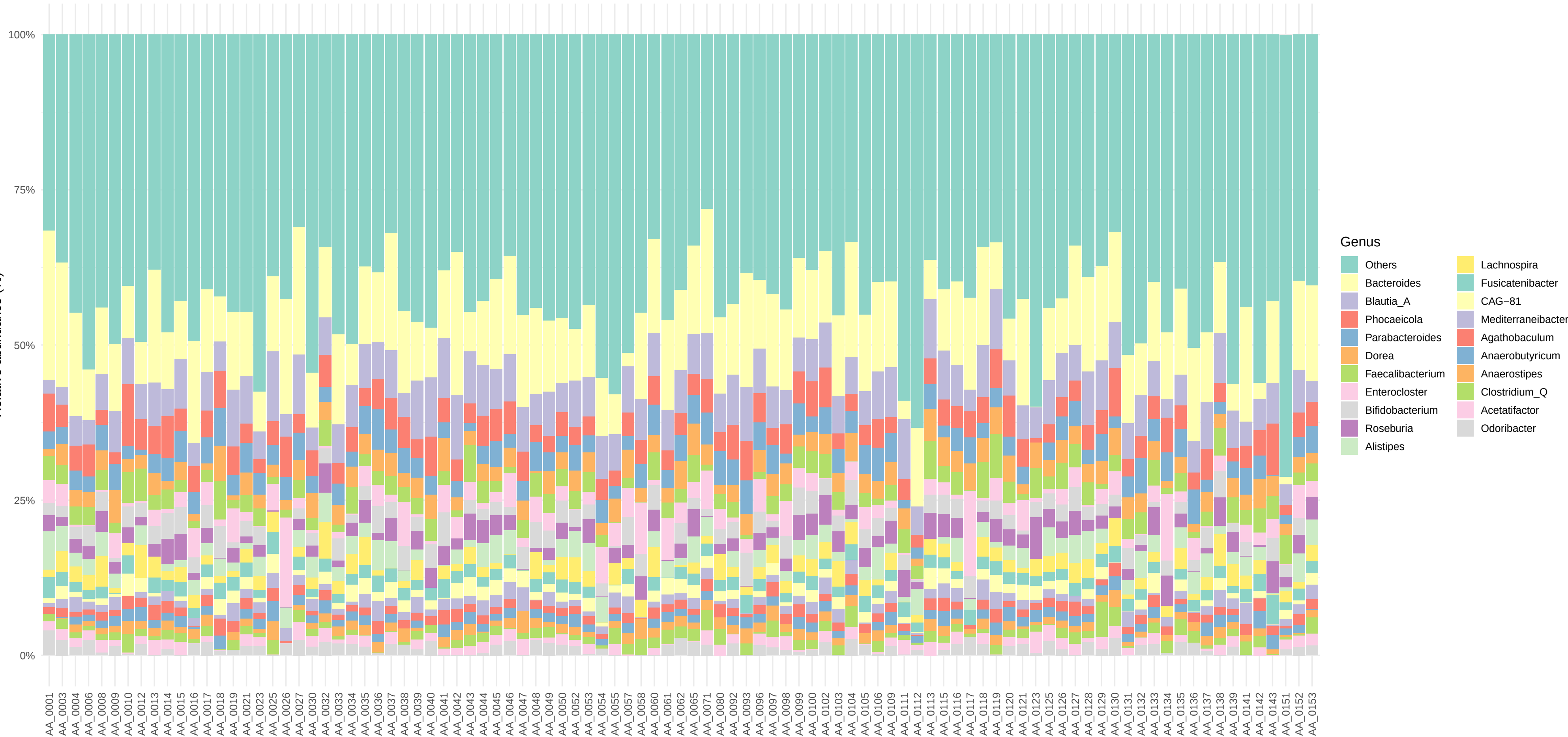
Relative Abundance at Genus Level
