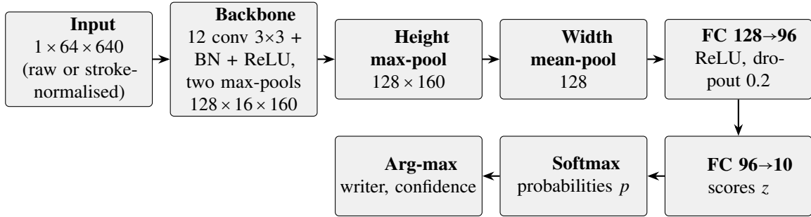
Figure 7. Architecture of the two writer classifiers. The backbone is that of the text recogniser; the head has 13 354 parameters. FC denotes a fully connected (linear) layer.
