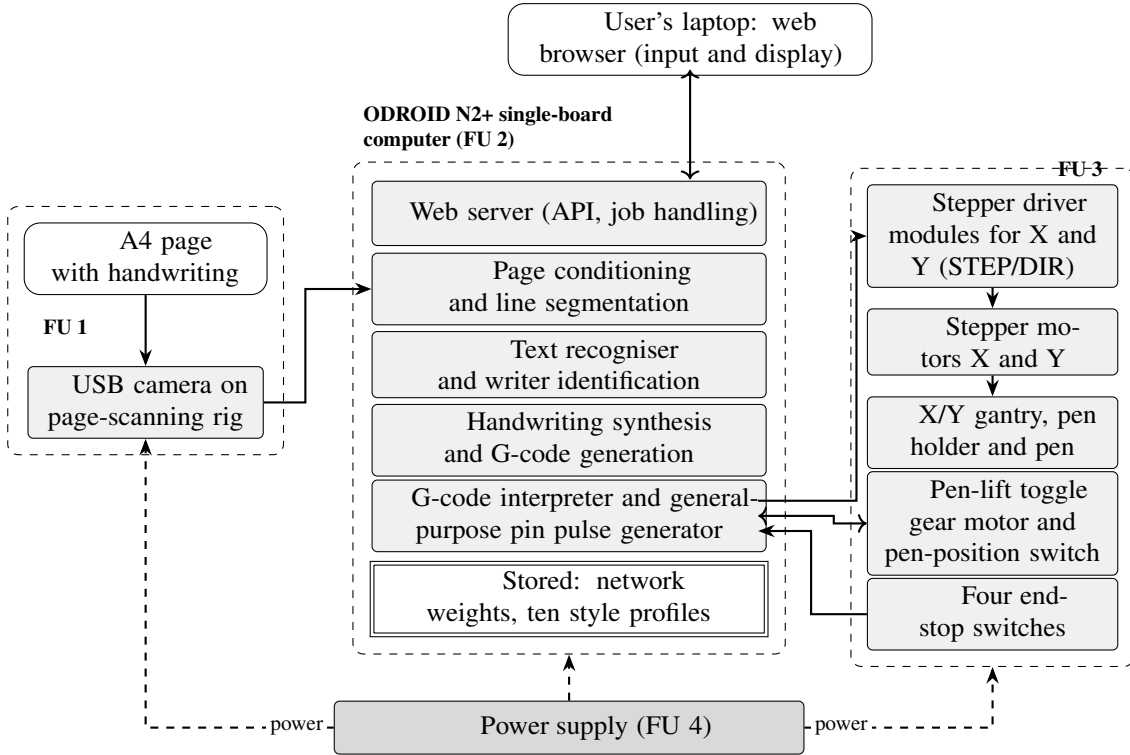
Figure 2. Hardware block diagram of the implemented system. Solid arrows show signals and data, dashed arrows show the power supply. FU numbers refer to the functional units of the project proposal.
