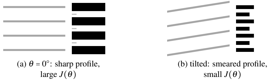
Figure 16. Principle of the projection-variance skew search. The bars on the right of each panel represent the row-sum profile of the ink. Aligned lines (a) give strong peaks and empty gaps and therefore a large variance, whereas a tilt (b) fills the gaps.
