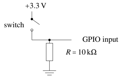
Figure 37. Switch input circuit as documented in the program comments; the closing current is 3.3\text{ V}/10\text{ k}\Omega = 0.33\text{ mA} . The origin of the 3.3 V (header pin) is inferred and [TO BE CONFIRMED BY STUDENT].
