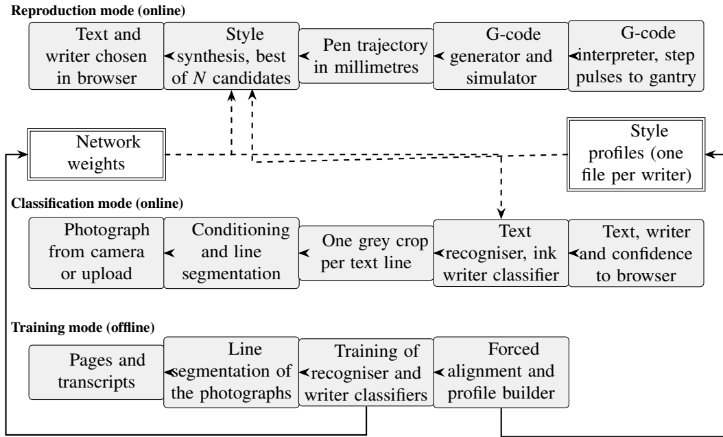
Figure 3. Software data flow of the three modes. Dashed arrows are reads from permanent storage, solid arrows between the training row and the two stores are writes. The same line-segmentation and recognition blocks serve classification, training and the judging of synthesised handwriting.
