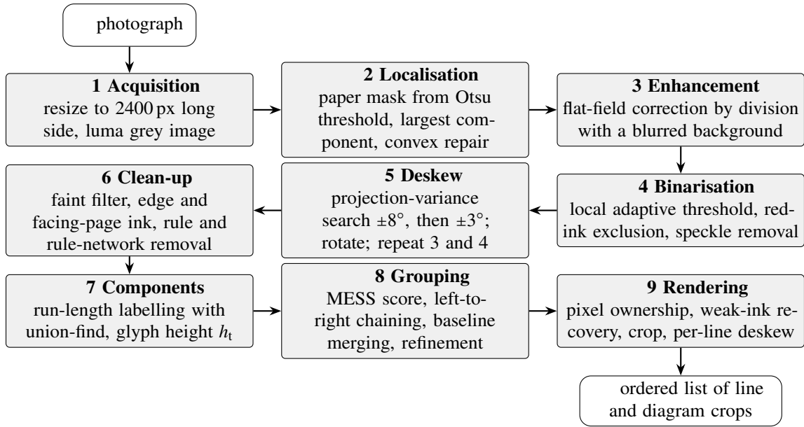
Figure 4. Flow diagram of the page-conditioning and line-segmentation block. The numbers correspond to the subsections of this subsection.
