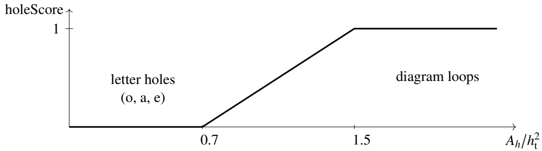
Figure 18. Score ramp of Equation 9. Holes that are smaller than 0.7h_t^2 are treated as letter counters and give a zero score, holes larger than 1.5h_t^2 give the maximum score.
