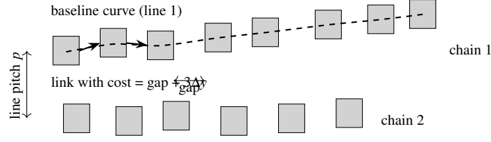
Figure 23. Schematic of the grouping of components into chains. Boxes are connected components, arrows are links that minimise Equation 10, and the dashed curve is the smoothed baseline of the upper chain.
