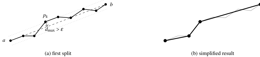
Figure 28. Douglas–Peucker simplification (schematic, tolerance exaggerated). (a) The vertex p_k with the largest distance d_{\max} from the chord ab lies outside the tolerance band (dotted) and splits the chain. (b) After recursion on both halves four of the original nine vertices remain.
