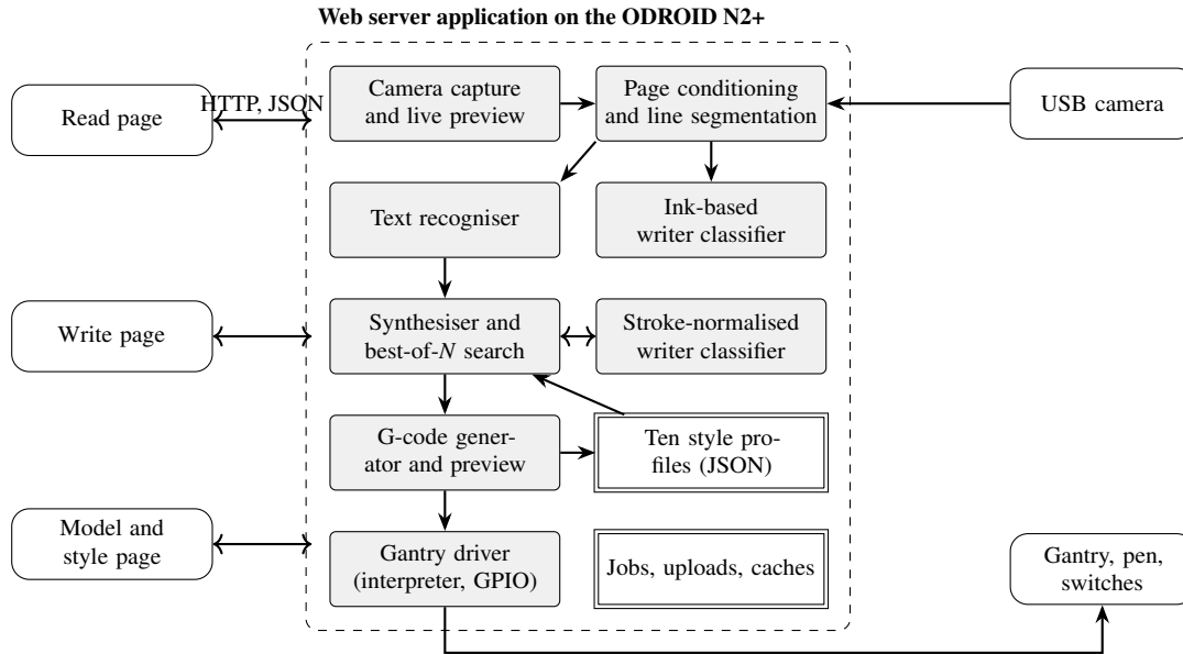
Figure 11. Software architecture. The three browser pages talk to one server application that links the blocks of Sections 3.3 to 3.9; the text recogniser also reads back every synthesised preview.
