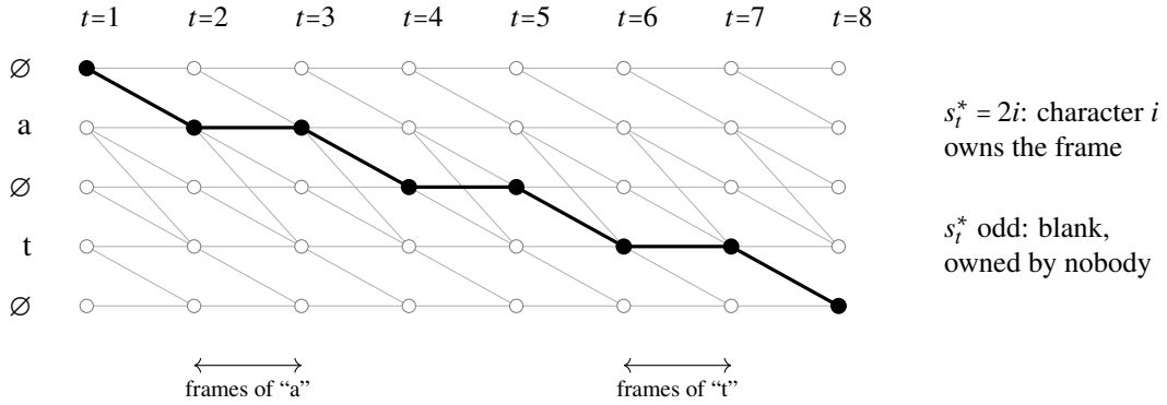
Figure 27. Forced-alignment lattice for the transcript “at” with T = 8 steps (cf. Figure 24). The thick path is the Viterbi path of Equation 40; only the frames on the row of a letter belong to that letter, so the spans are narrow.
