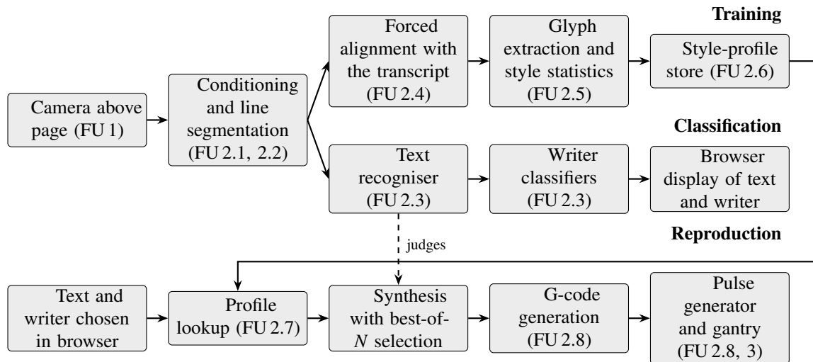
Figure 1. Block diagram of the chosen concept. Solid arrows show the flow of data; the dashed arrow shows that the recogniser and writer classifier also judge the candidates in the synthesis block. Functional-unit numbers of the proposal are in brackets. Training is performed offline and is not part of the browser interface.
