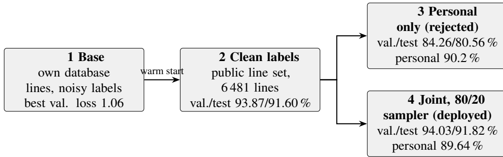
Figure 26. Staged training recipe of the text recogniser with the character accuracies (public validation and test sets, and personal validation; see Table 7 for the caveats).
