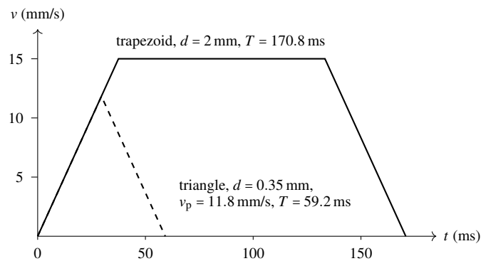
Figure 36. Velocity profiles of Equation 62 for a = 400 \text{ mm/s}^2 and v = 15 \text{ mm/s} : a 2 mm move is trapezoidal (solid); the usual 0.35 mm segment is triangular (dashed) and never reaches the cruise speed.
