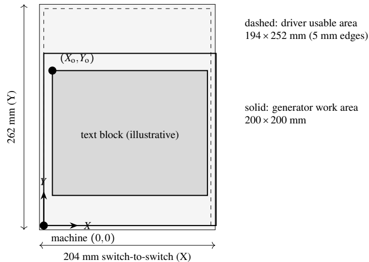
Figure 33. Coordinate frames drawn to scale. The machine frame has its origin 5 mm inside the minimum switches; the generator places the text block with its top-left corner at (10, 180) mm inside a 200 × 200 mm work area, and the driver clamps all targets to its calibrated usable area of 194 × 252 mm. The extent of the text block is illustrative.
