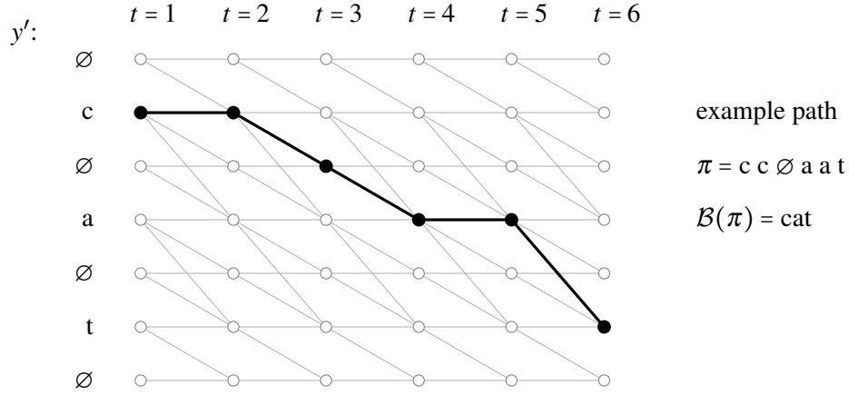
Figure 24. CTC lattice for the word “cat” with T = 6 steps. The rows are the positions of the blank-augmented label y' ; thin lines are the allowed transitions of Equation 24 (stay, advance, and skip over a blank between different letters). The thick path is one of the many paths that collapse to the word.
