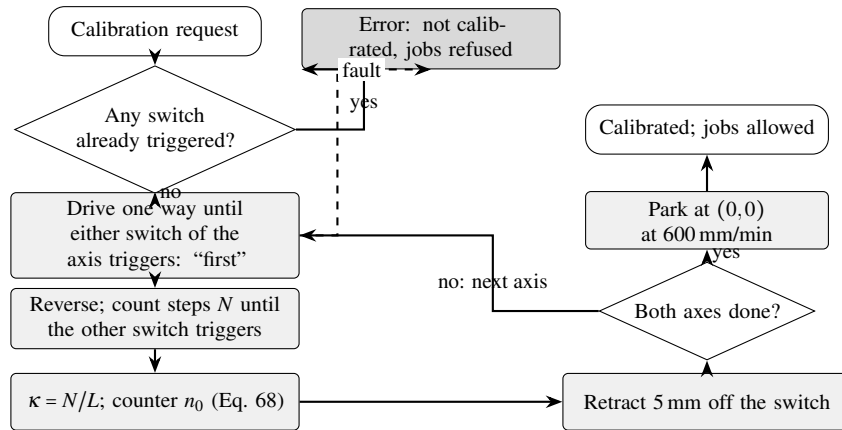
Figure 10. Flow chart of the calibration; the left column runs for each axis in turn (X, then Y). A triggered switch at the start, an unexpected switch or more than 200 000 steps without a trigger is a fault.
