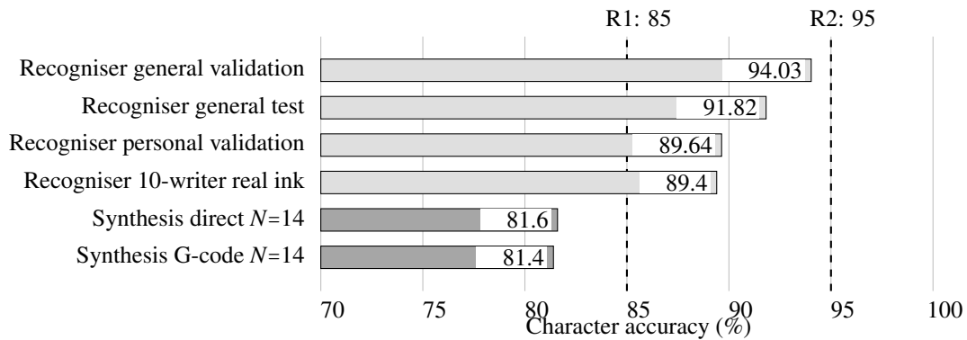
Figure 12. Established character accuracies against the targets of R1 and R2. Light bars: recogniser on the general benchmark and on personal or real-ink data (optimistic splits). Dark bars: synthesised text read by the search judge (circular). The axis starts at 70%.
