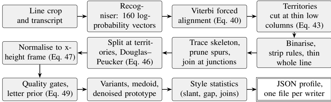
Figure 8. Flow chart of the offline style-profile builder: alignment (top), glyph extraction (middle) and profile assembly (bottom).
