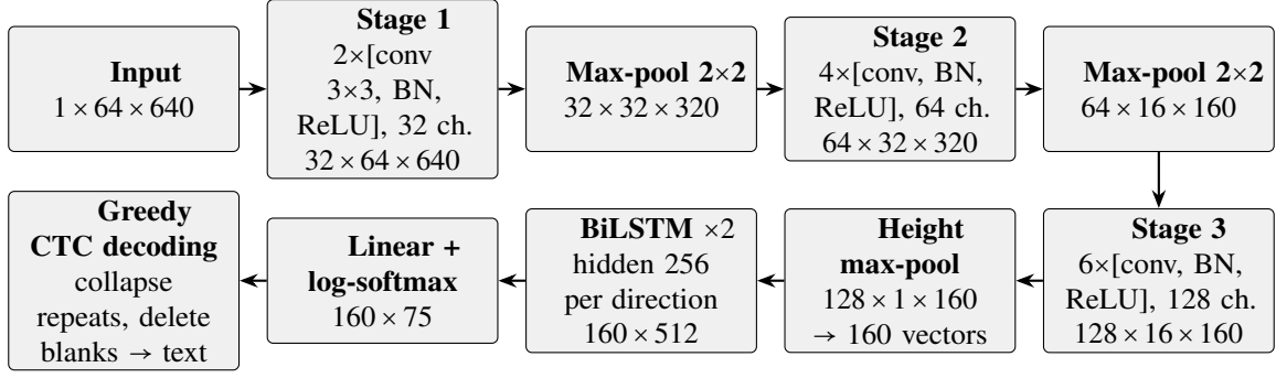
Figure 6. Architecture of the text recogniser. Tensor shapes are channels \times height \times width for the convolutional part and time steps \times features for the recurrent part; BN denotes batch normalisation.
