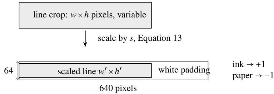
Figure 19. Pre-processing of a line crop. The crop is scaled uniformly, left-aligned on a white canvas and normalised to the range [-1, 1] (Equation 14).
