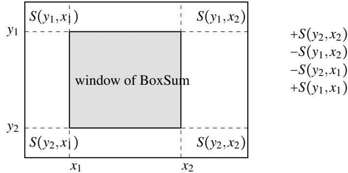
Figure 13. The four-corner rule of the summed-area table. Each table entry S(y, x) is the sum of all pixels above and to the left of (y, x) (measured with the vertical axis pointing down), so the shaded window sum follows from four entries (Equation 4).
