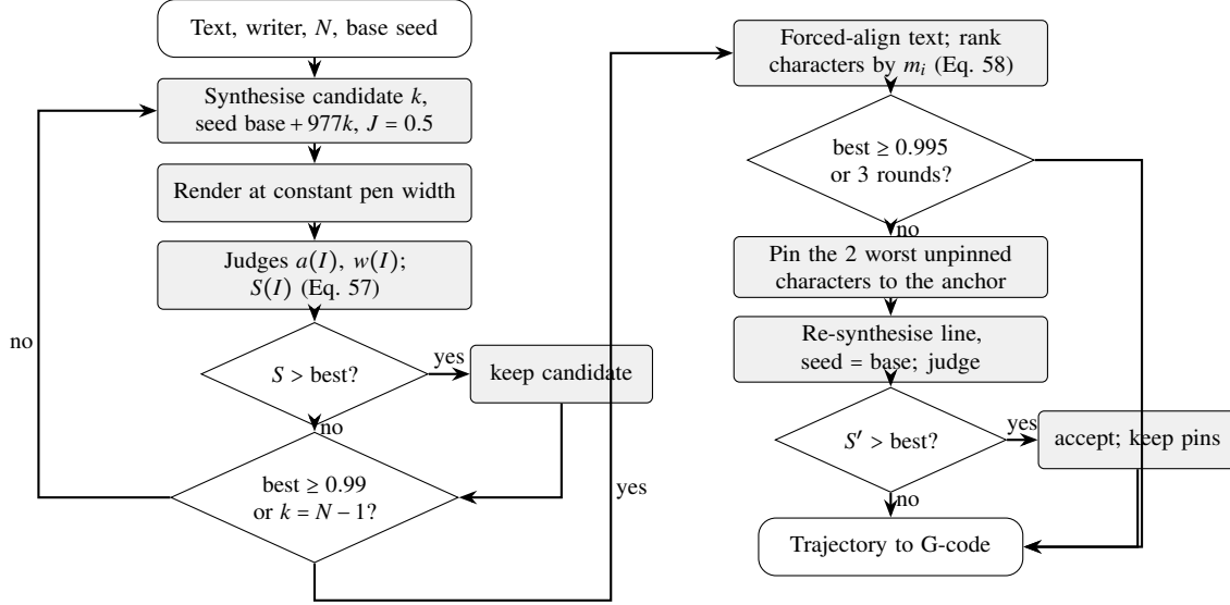
Figure 9. Flow chart of the joint best-of- N search: the search over N candidates (left) and the repair pass (right). A repair round ends after acceptance or rejection and the next round starts from the best candidate; when its test is satisfied the repair loop exits to the output.
