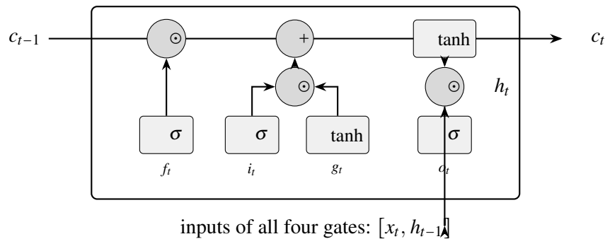
Figure 20. Schematic of an LSTM cell (Equation 18). The memory line c_t at the top is changed only by the forget gate (multiplication) and the input gate (addition), which allows information to travel over many time steps.
