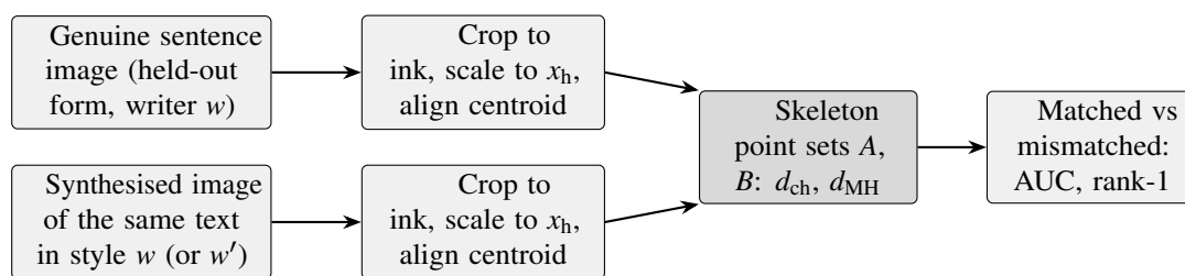
Figure 38. Overlay test of qualification test 1: both images are normalised in the same way and matched writer pairs are compared with mismatched pairs.
