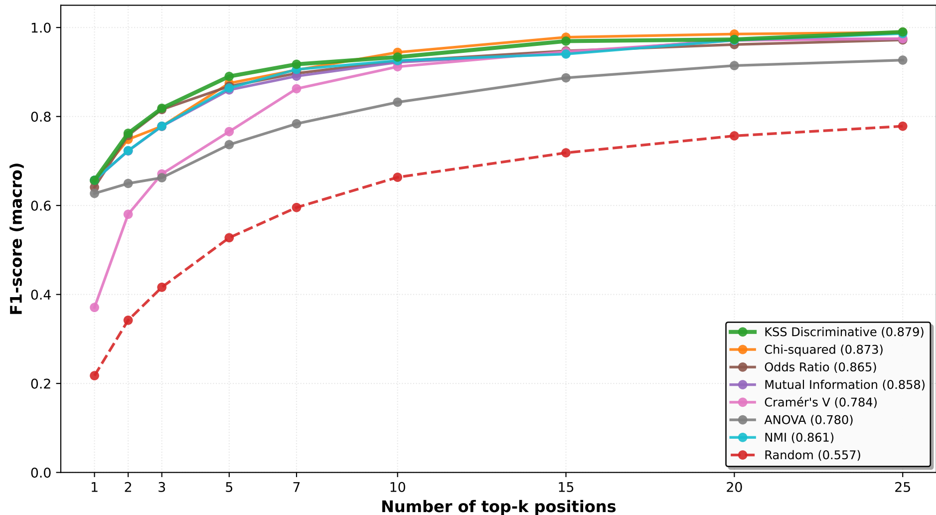
Classification Performance by Discriminative Metric
