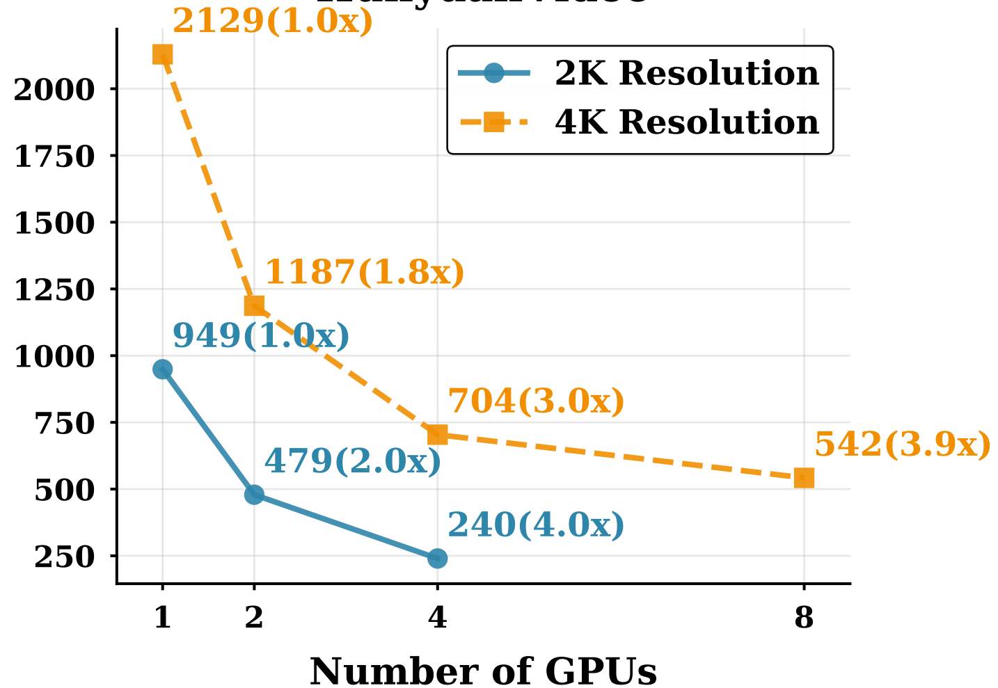
HunyuanVideo
