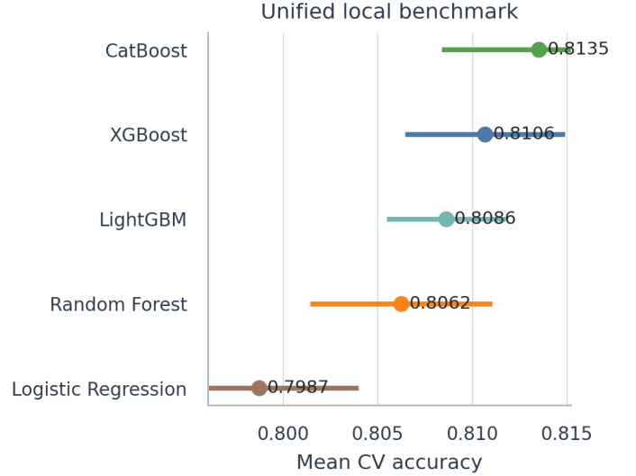
Fig. 4. Mean CV accuracy under the unified benchmark. Boosting clearly dominates the task.
