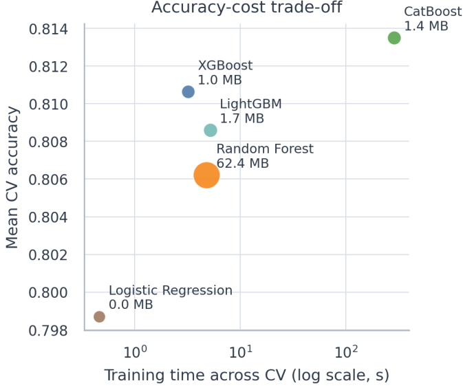
Fig. 5. Accuracy-cost trade-off. CatBoost is strongest locally, while XGBoost is the most attractive speed-performance compromise.
