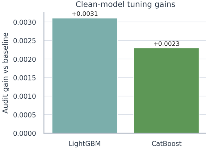
Fig. 8. Audited tuning gains for the clean LightGBM and CatBoost search tracks preserved in the local experiment logs.
