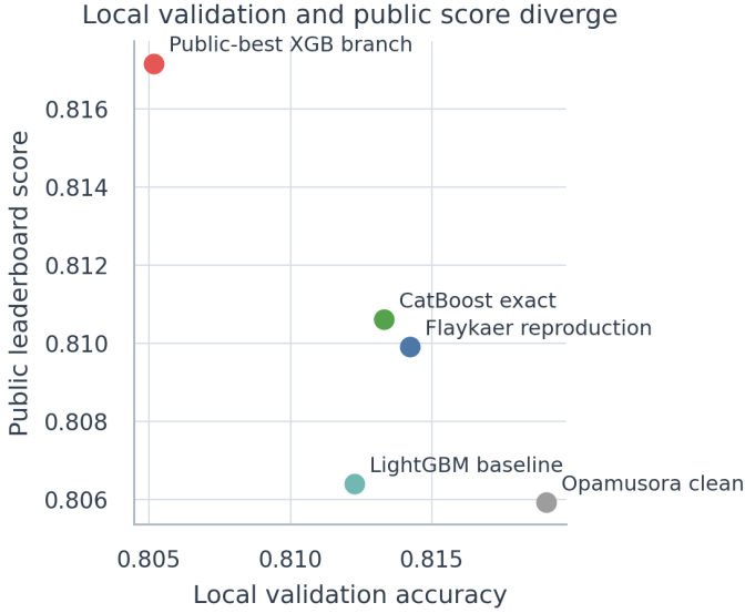
Fig. 9. Local validation does not monotonically predict public leaderboard score. This is why the report emphasizes validation design and ablation rather than public-score chasing alone.
