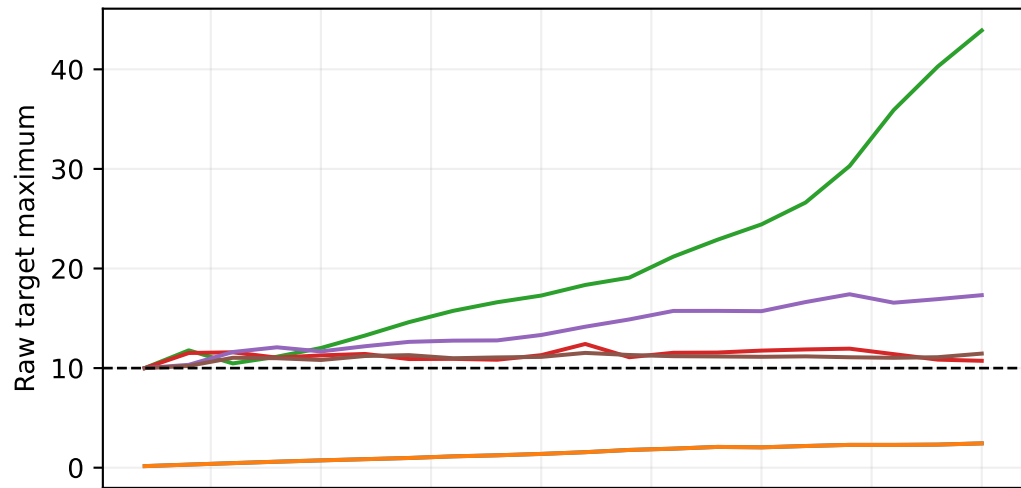
Seed 0: raw TD target before clipping
