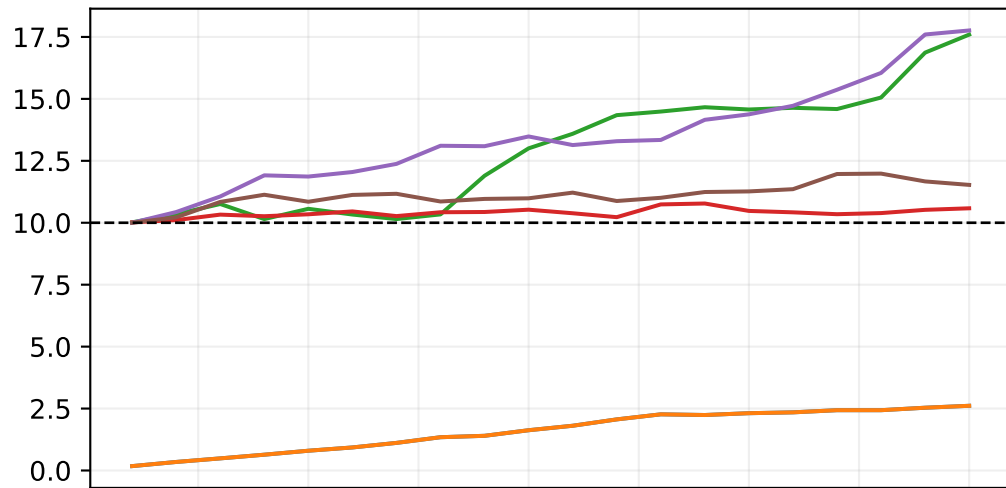
Seed 1: raw TD target before clipping
