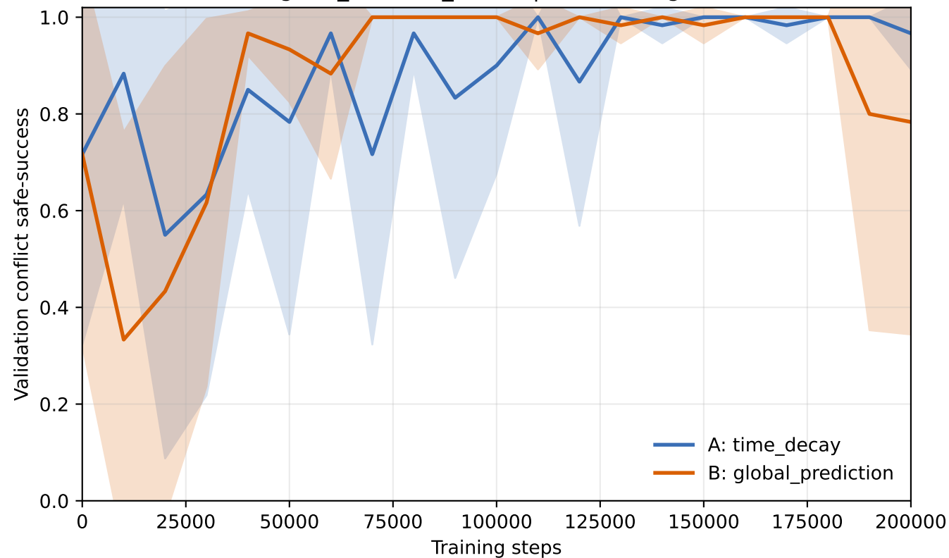
irregular_workcell_91702 | full learning curve
