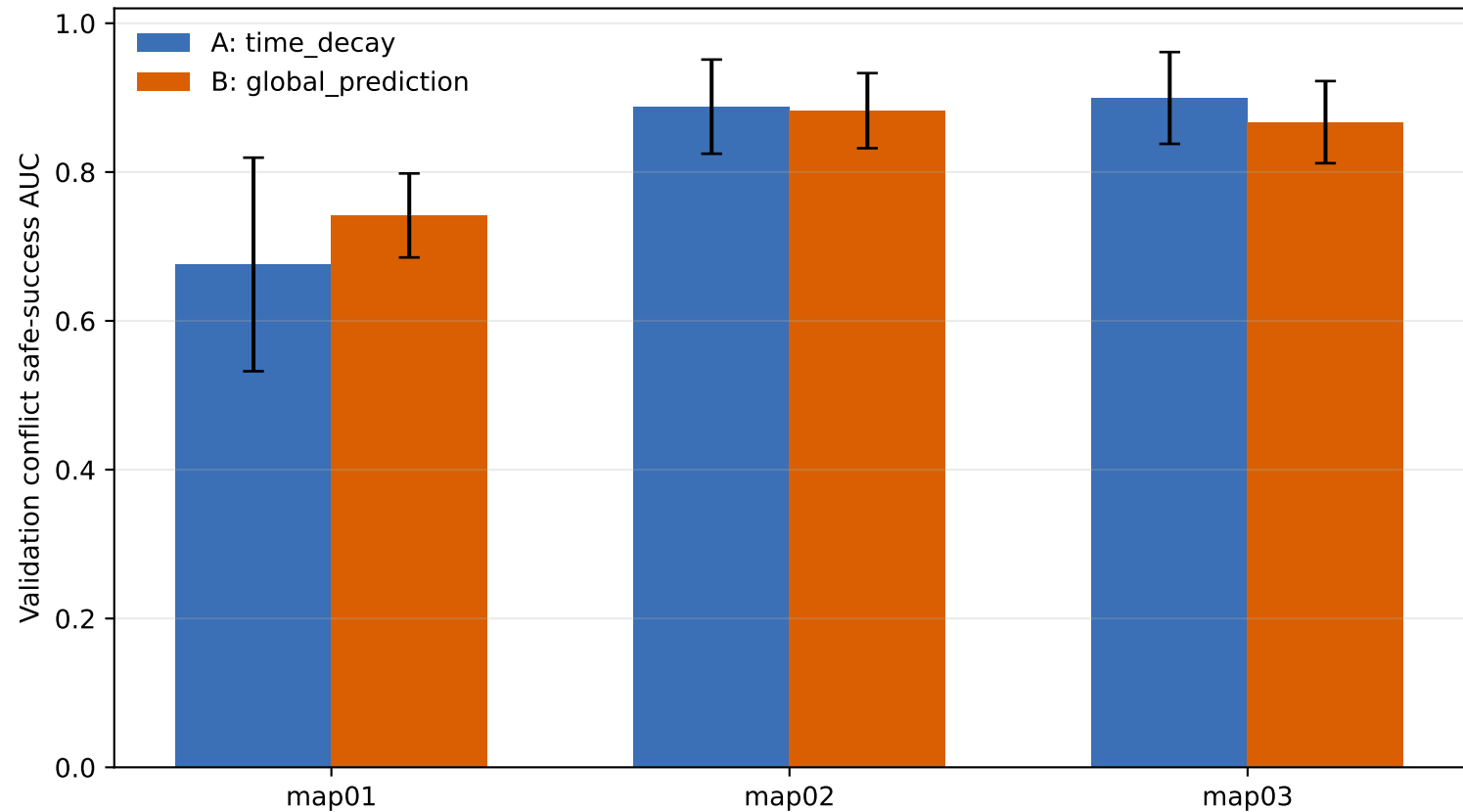
Five-seed validation AUC (mean \pm std)
