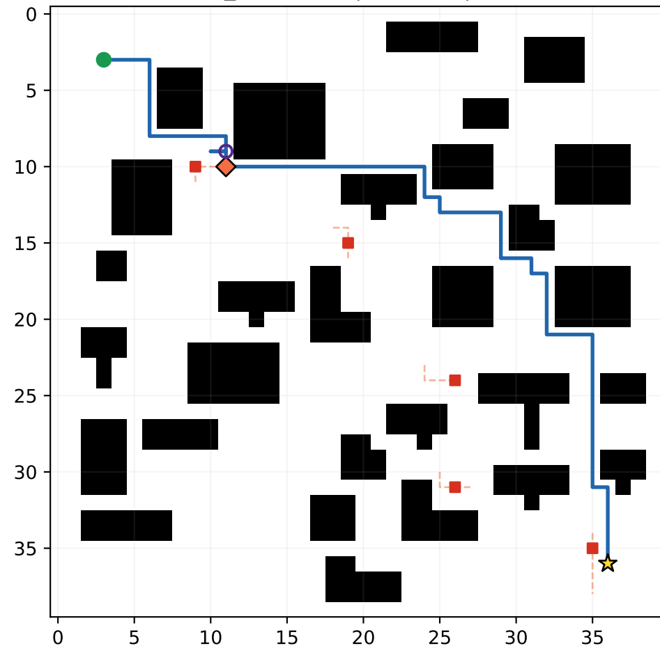
B: global_prediction | success | steps=68
