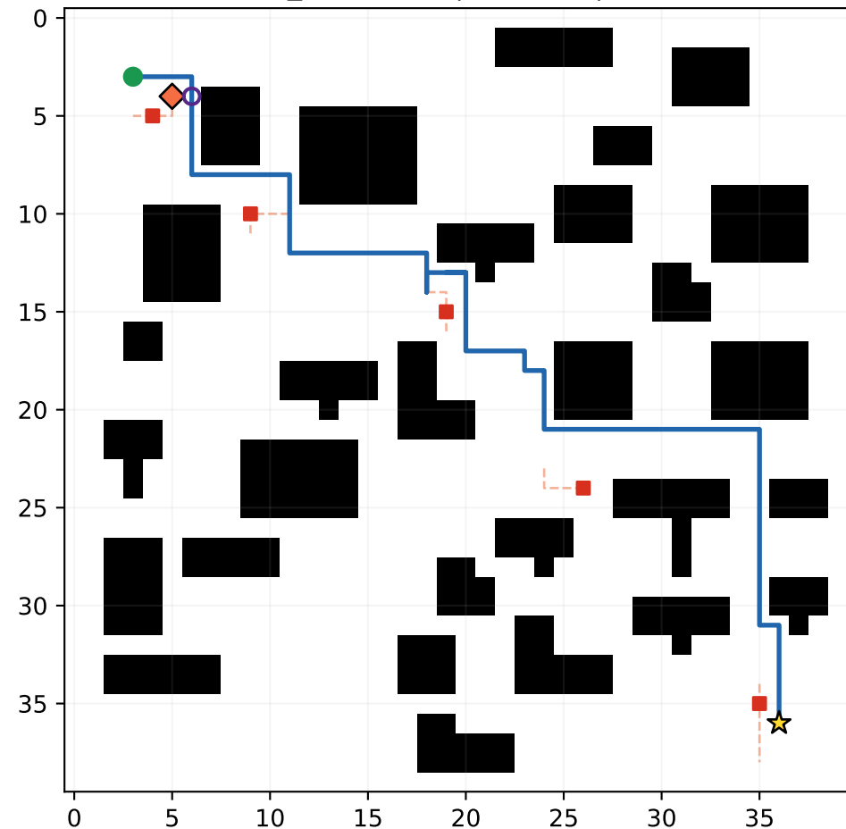
B: global_prediction | success | steps=73
