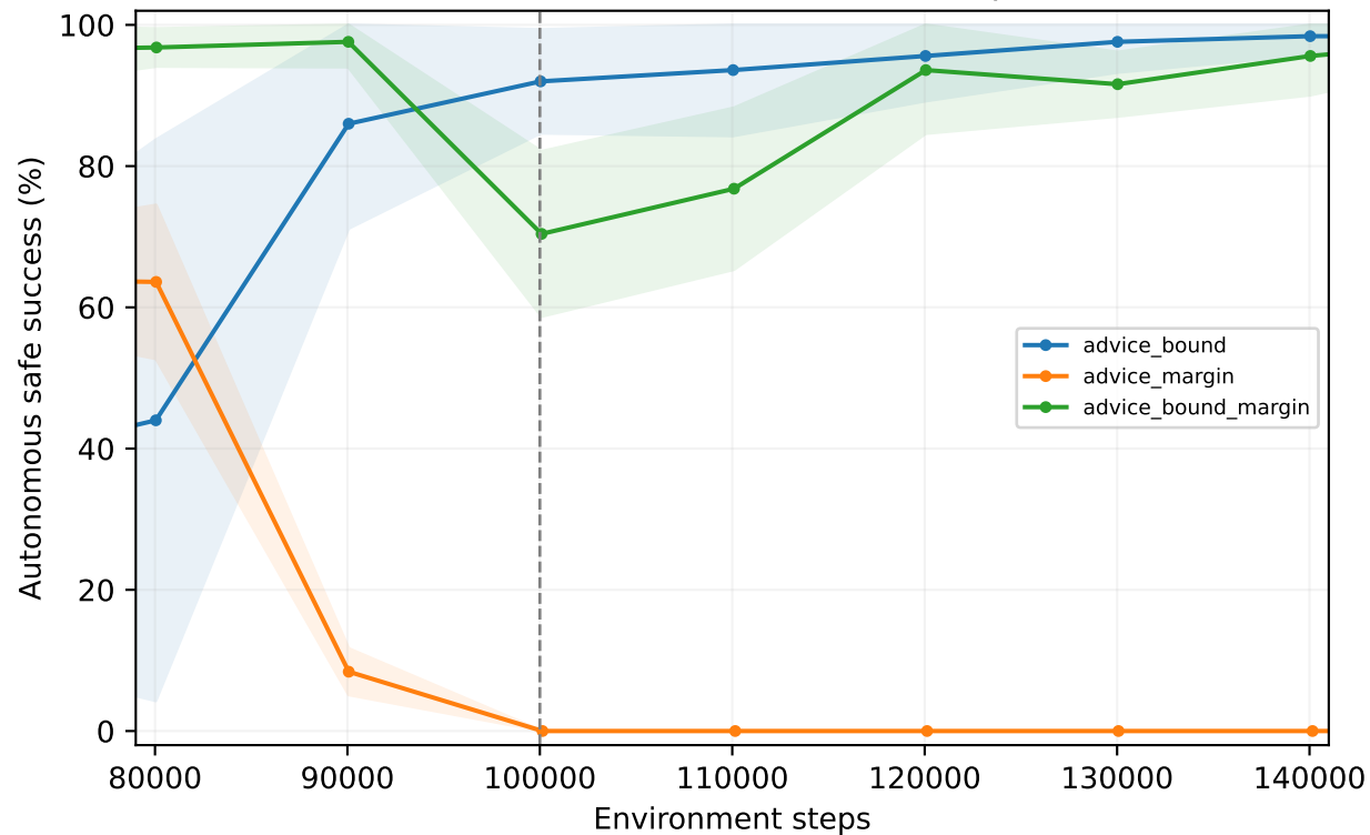
Teacher withdrawal: mean and sample SD
