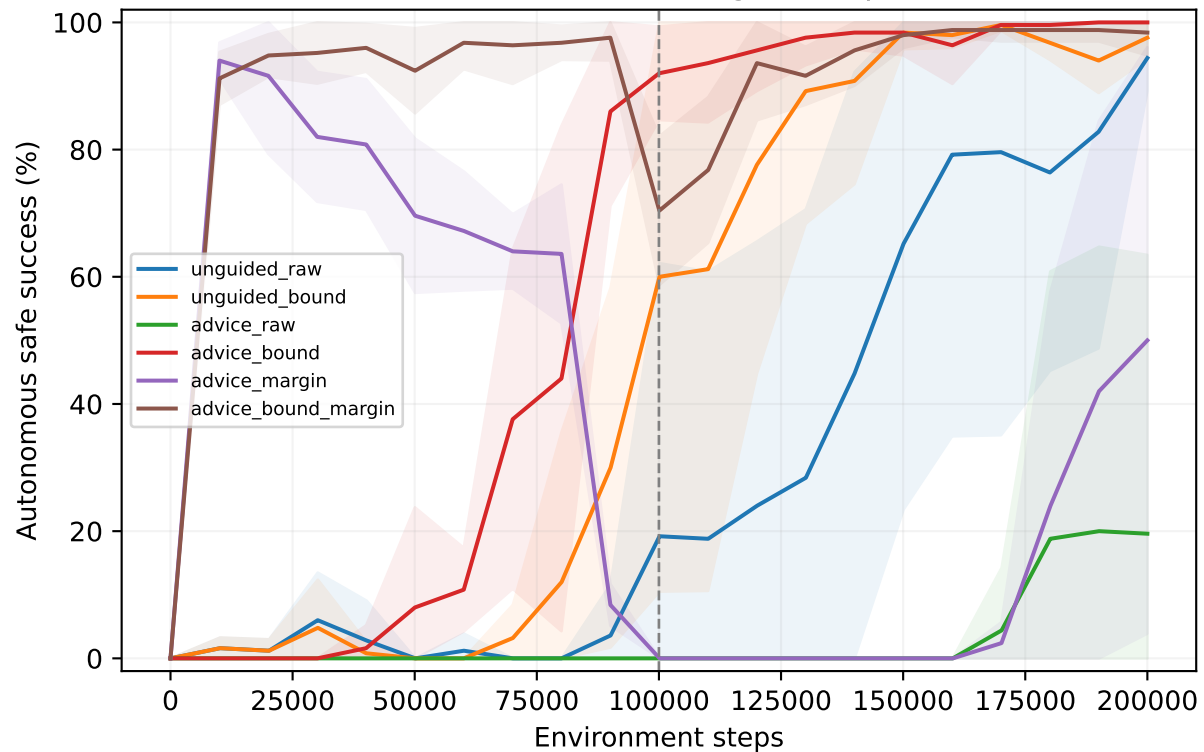
Five-seed mean; shading = sample SD
