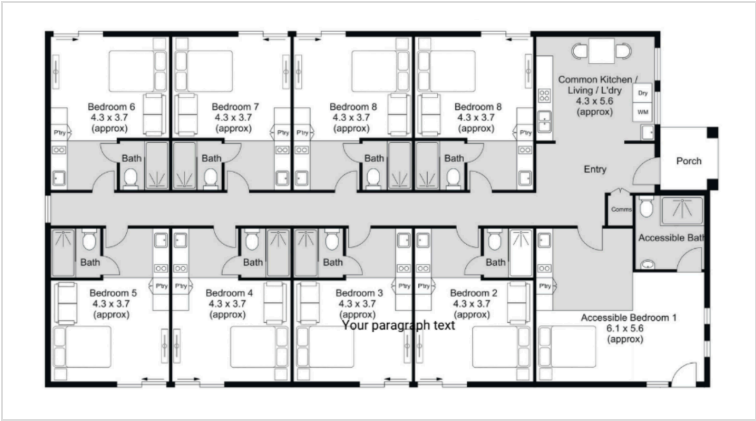
EXAMPLE FLOOR PLAN — 9 BEDROOMS. FINAL LAYOUT VARIES PER BLOCK.
