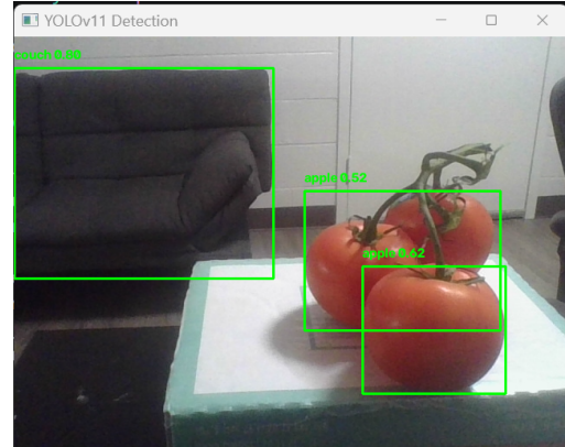
(b) Wrong: tomatoes detected as apple.
