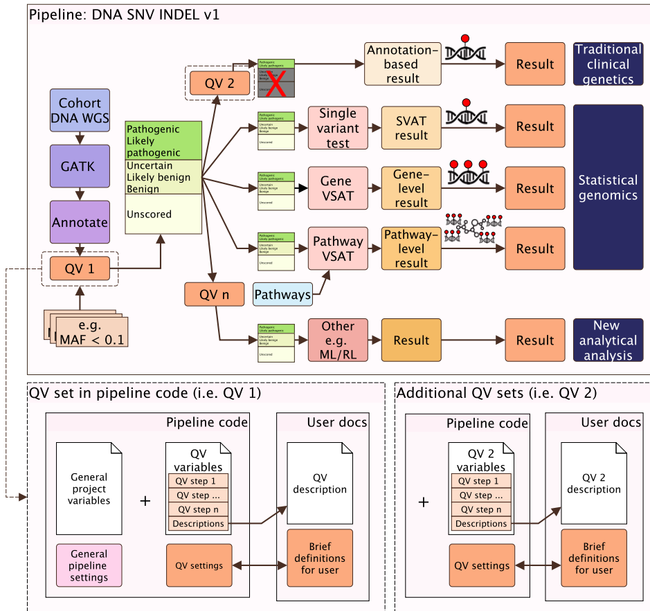
Fig. 1. Summary of the QV application for a WGS pipeline. QV1 and QV2 are applied as sequential protocol steps. In this example, QV2 differs from QV1 by retaining only likely/pathogenic variants (indicated by a red X). The QV file loaded by the analysis pipeline comprises a description field (optional) and a variables field (mandatory). The QV criteria may be distributed across multiple pipeline steps.
