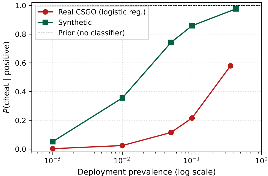
Base-rate effect on positive predictive value
