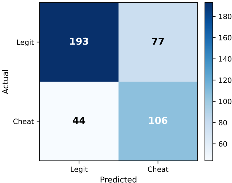
CSGO test-set confusion matrix (logistic regression session model)
