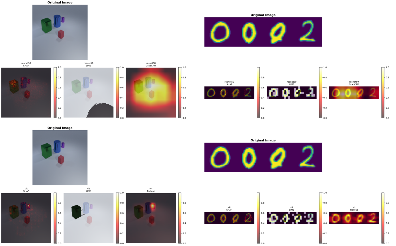
Fig. 1. Visual comparison of post-hoc methods. Top Left: ResNet50 on CLE4EVR. Top Right: ResNet50 on MNMath. Bottom Left: ViT on CLE4EVR. Bottom Right: ViT on MNMath.
