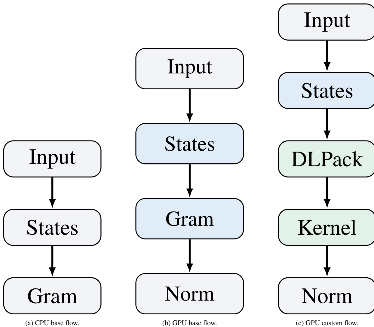
Figure 2: Horizontal comparison of backend pipelines referenced in the HPC architecture section.
