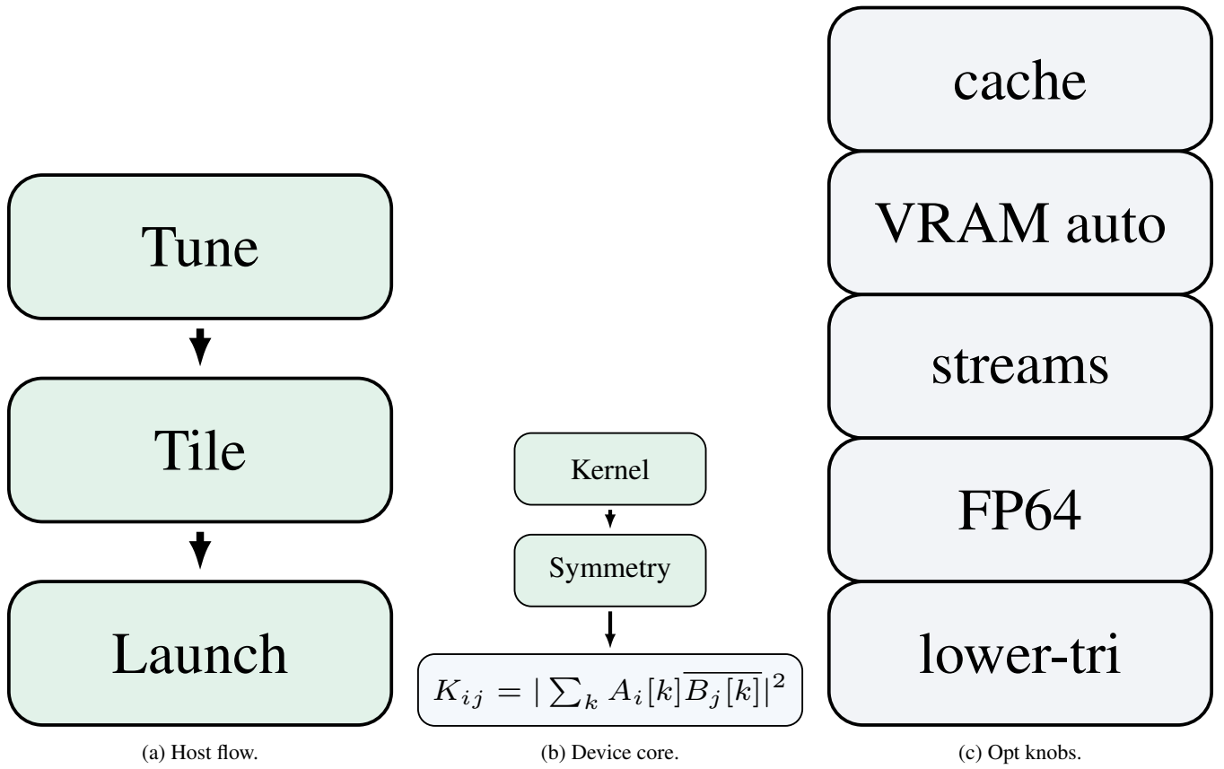
Figure 3: Kernel construction in GPU custom , organized across three full-width elements: host orchestration, device kernel core, and optimization controls.
