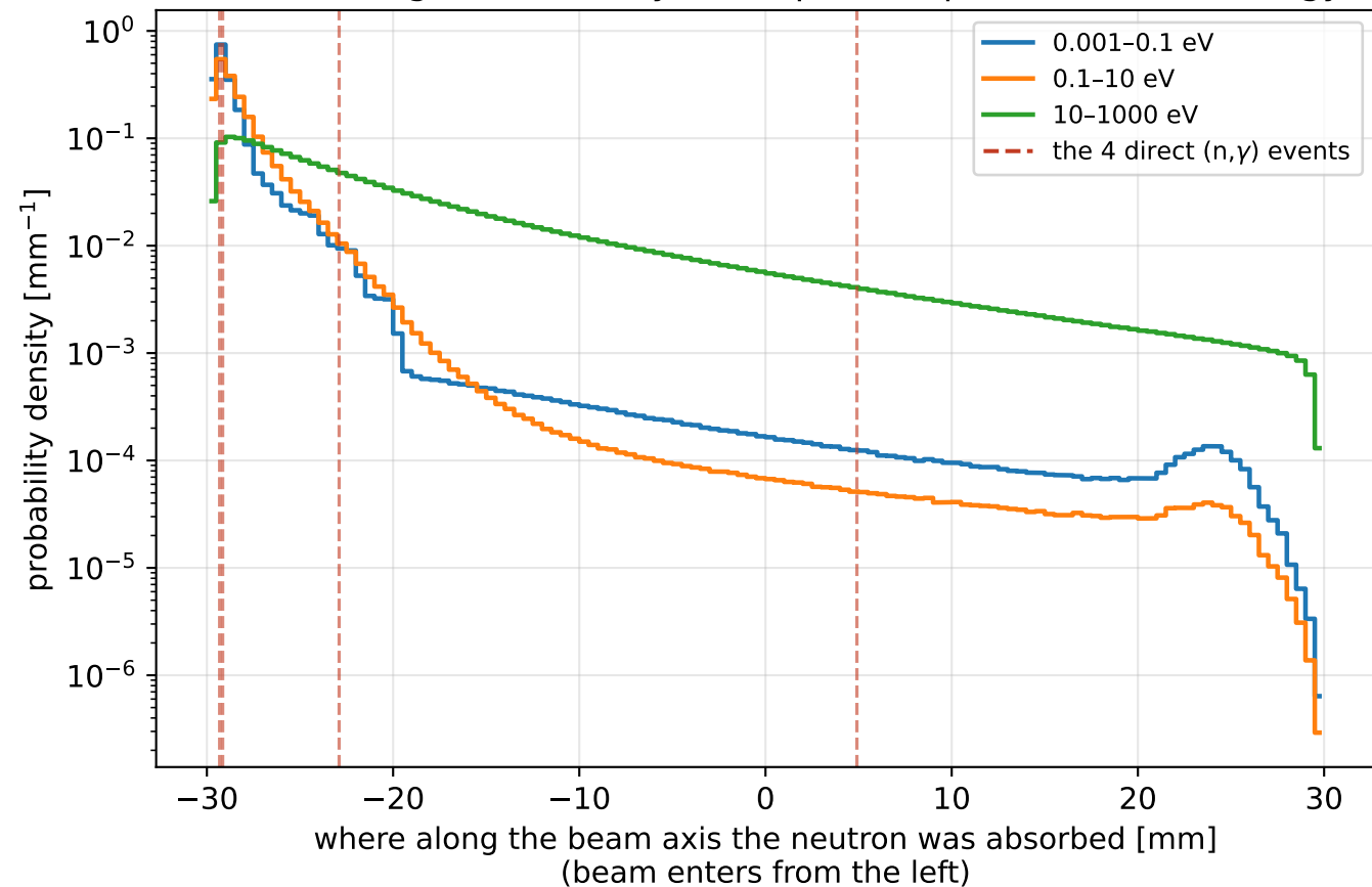
Self-shielding seen directly: absorption depth vs neutron energy
