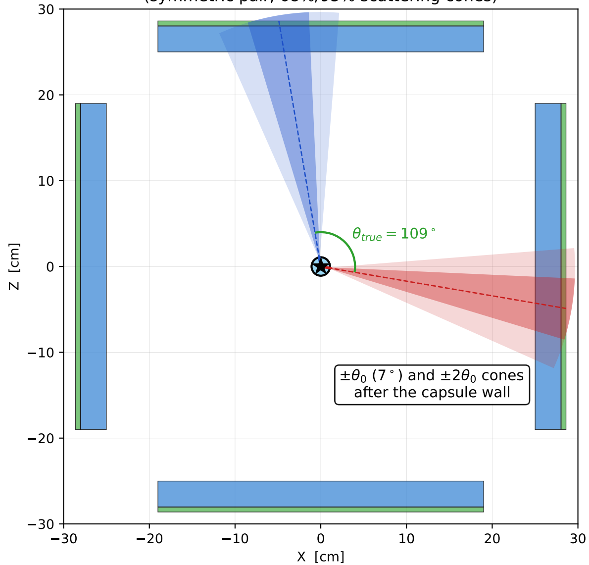
Where each track can land after the wall (symmetric pair, 68%/95% scattering cones)
