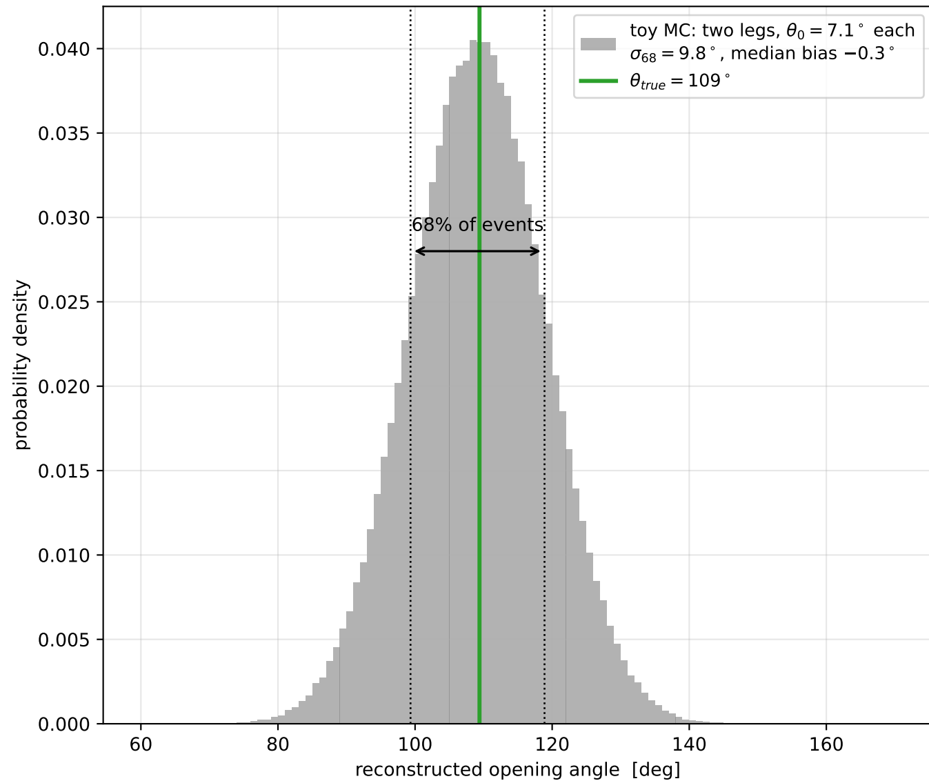
What one fixed true angle becomes (Geant4 full-spectrum value: \sigma_{68} = 12.5 - 15.5^\circ )
