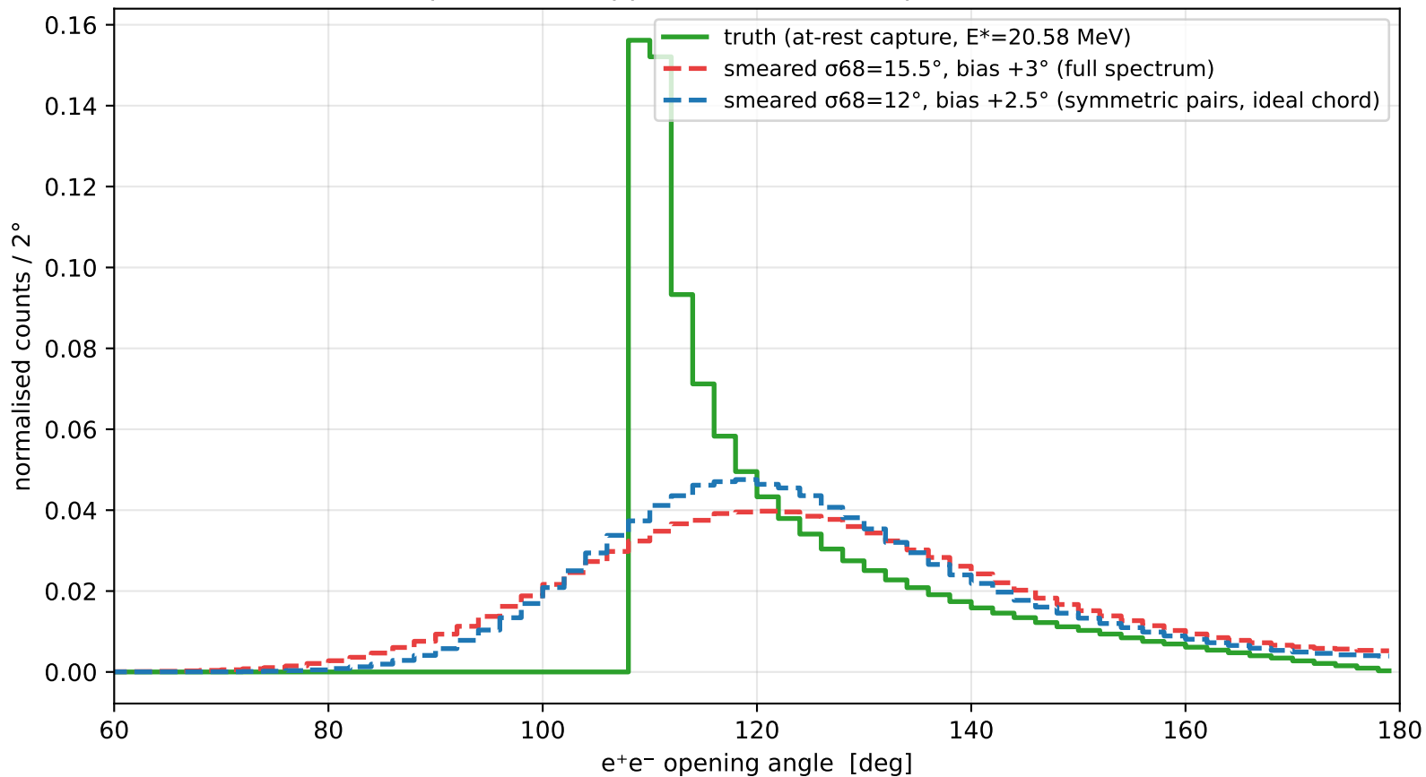
X17 opening-angle peak dilution by the measured resolution (acceptance not applied; Gaussian-response illustration)
