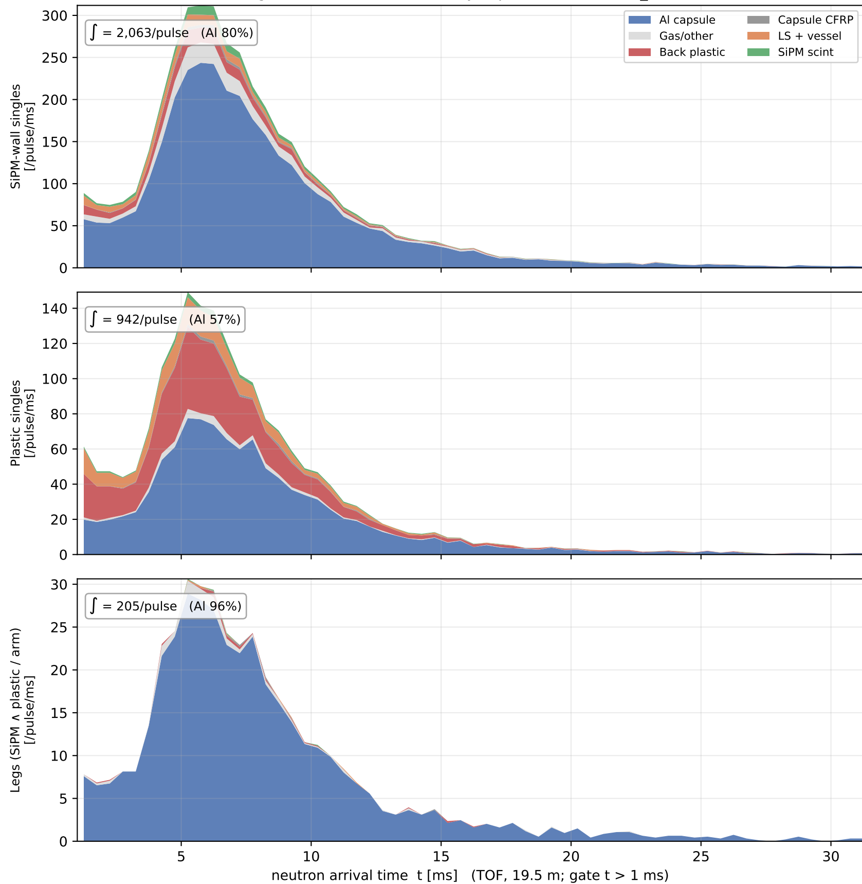
Thermal-gate rates vs arrival time, by capture source (sim, _2cm, 0.5 MIP)
