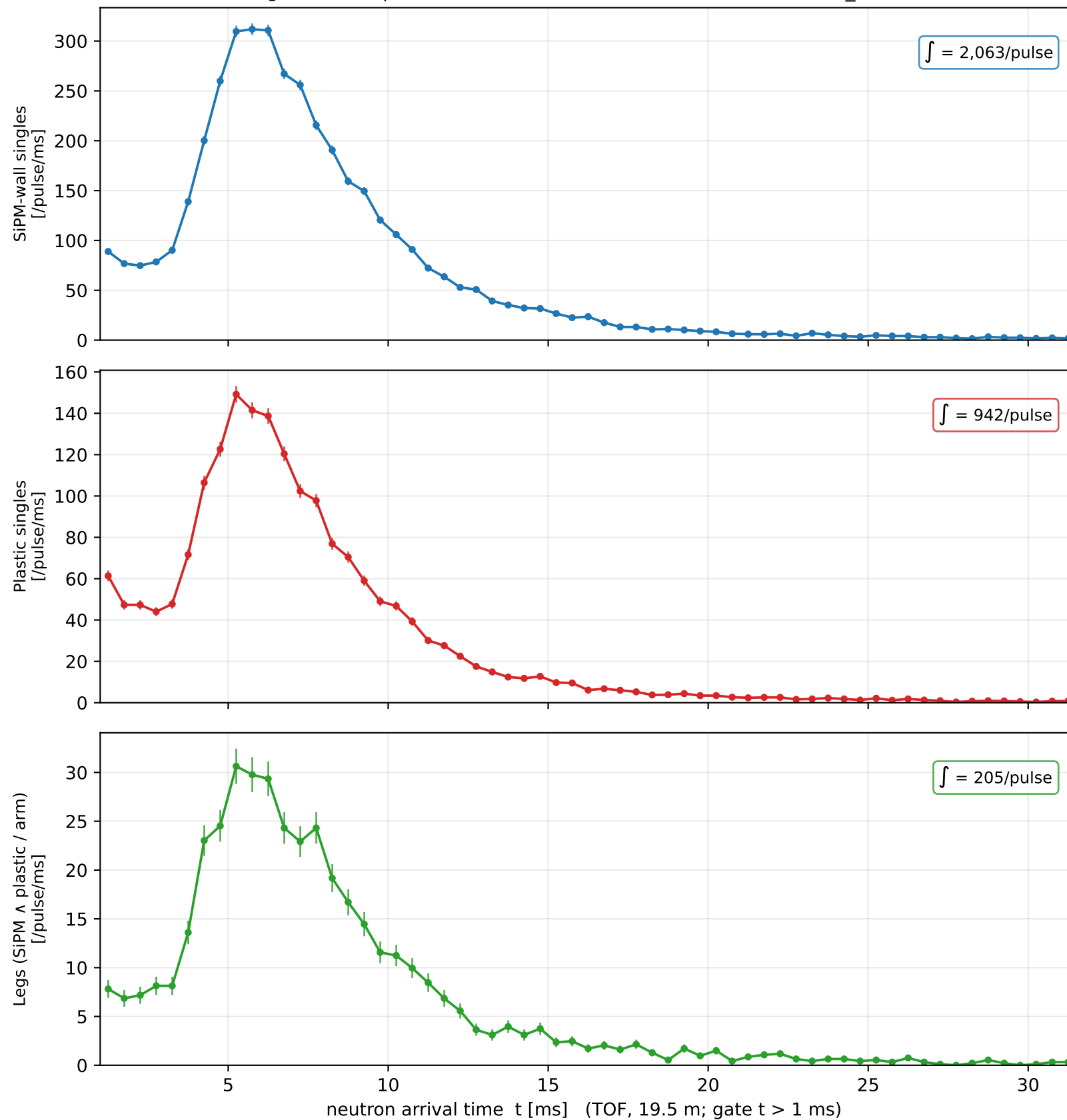
Thermal-gate SiPM / plastic / coincidence rates vs arrival time (sim, _2cm, 0.5 MIP)
