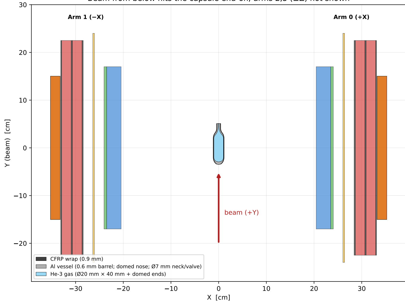
MX17 Geometry — Side View (XY plane) Beam from below hits the capsule end-on; arms 2,3 ( \pm Z ) not shown
