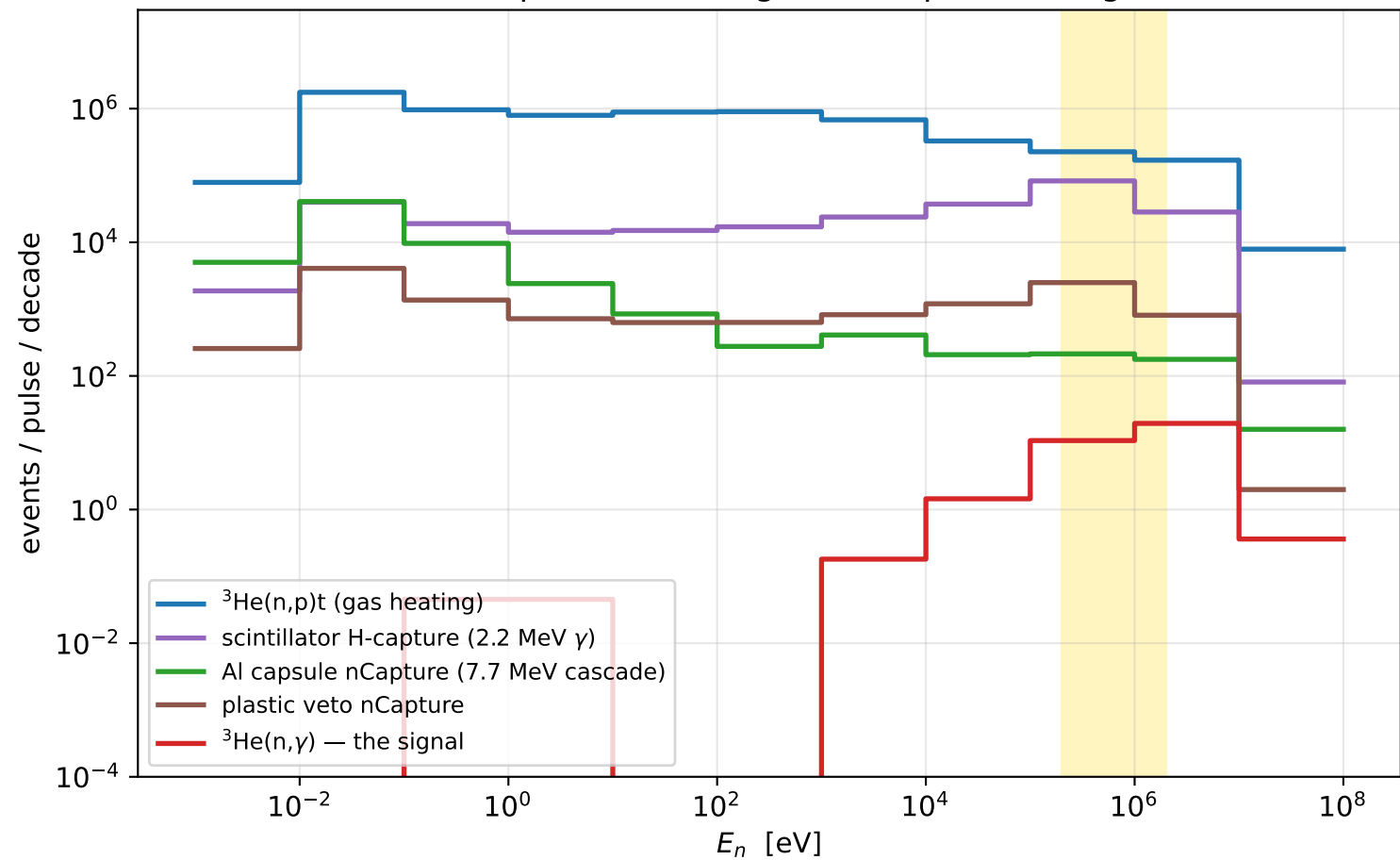
Neutron fate per decade: signal vs capture backgrounds
