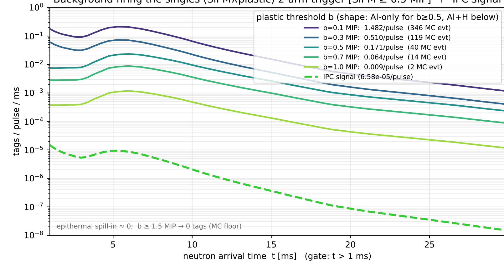
Background firing the singles (SiPM \wedge plastic) 2-arm trigger [SiPM \geq 0.5 MIP] + IPC signal
