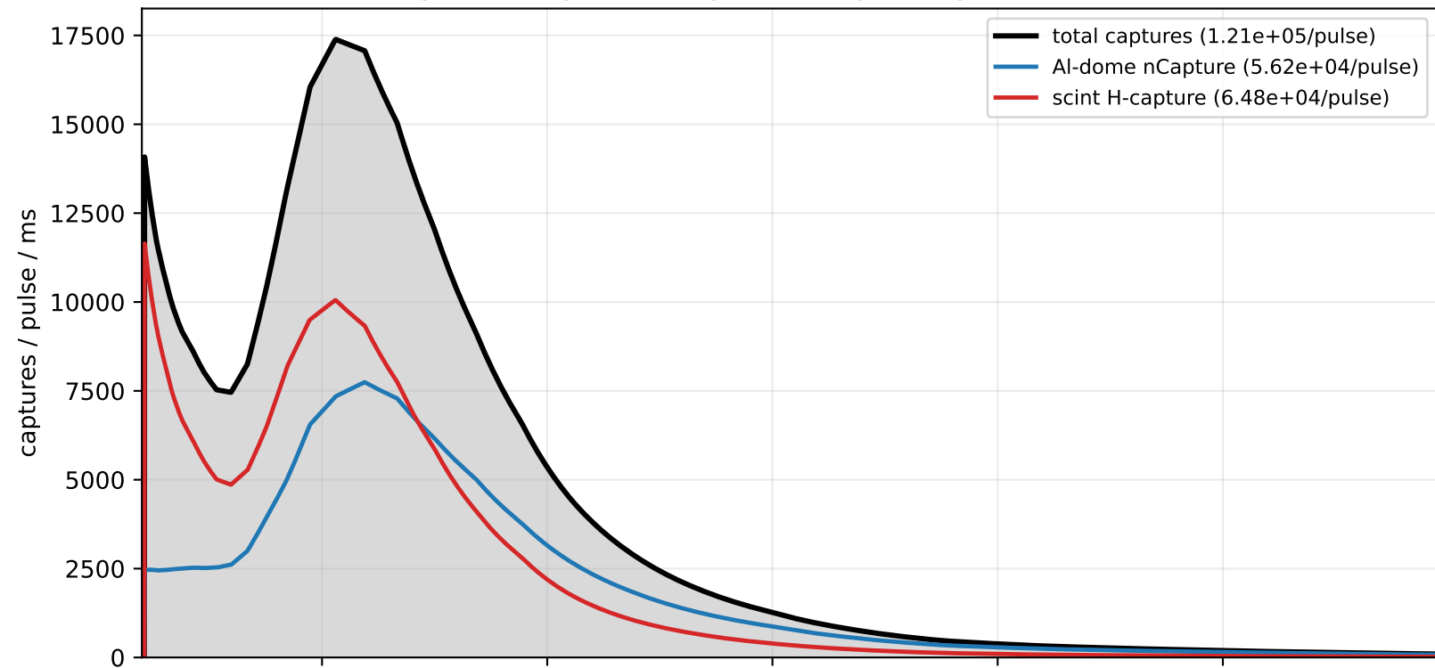
Background firing the singles (SiPM \wedge plastic) 2-arm trigger [SiPM \geq 0.5 MIP] + IPC signal
