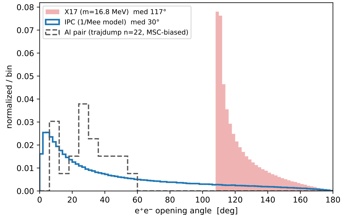
Truth opening-angle distributions (infinite-stats shapes)
