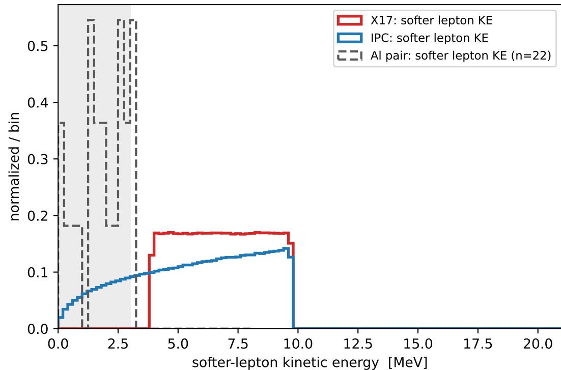
Individual-lepton energy (a possible track-level handle)
