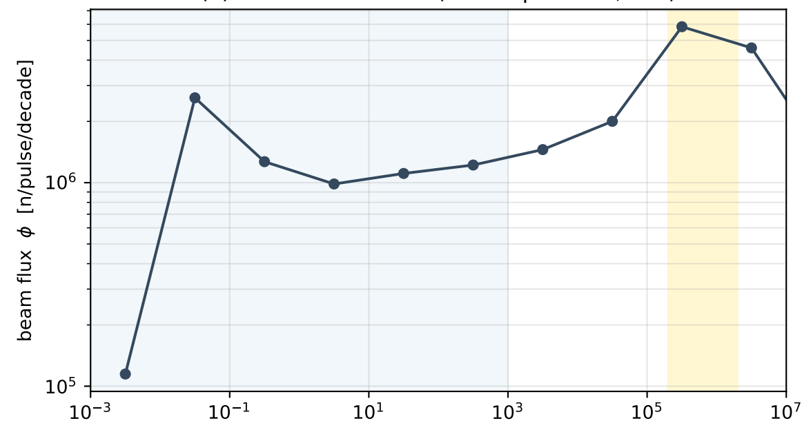
(a) total neutron flux (EAR2 spectrum, sim)
