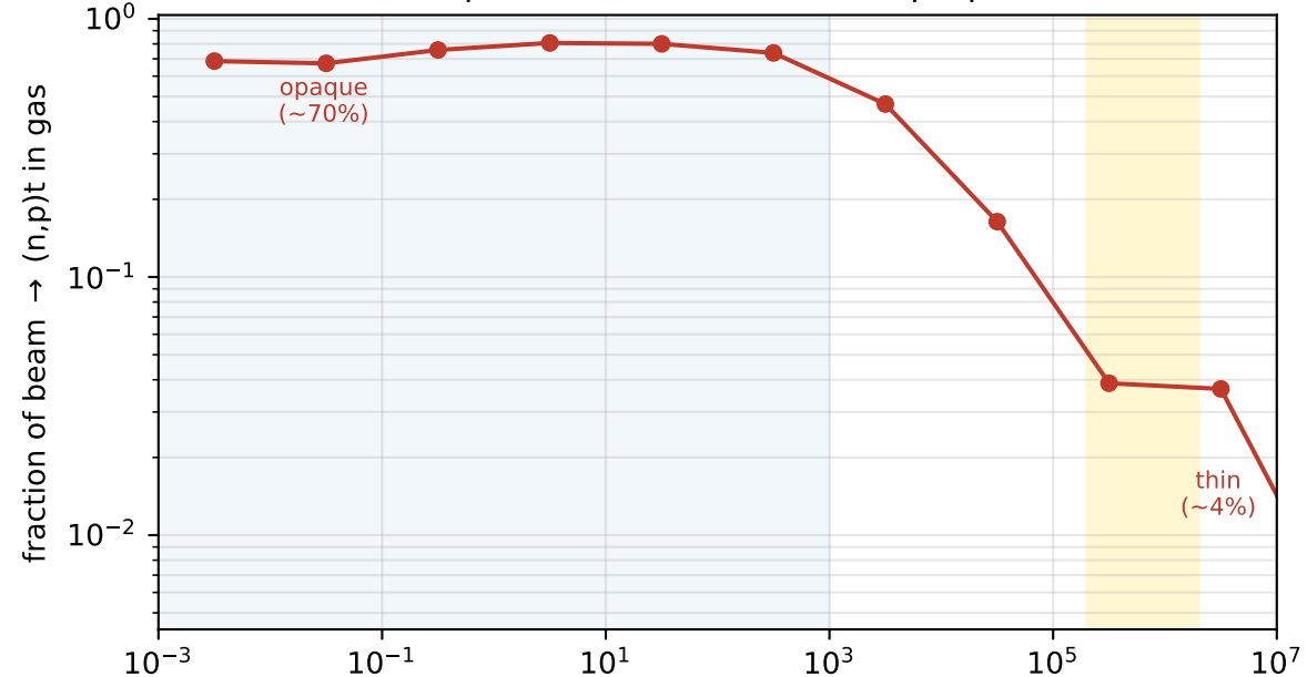
(b) breakup (interaction) fraction: opaque \rightarrow thin
