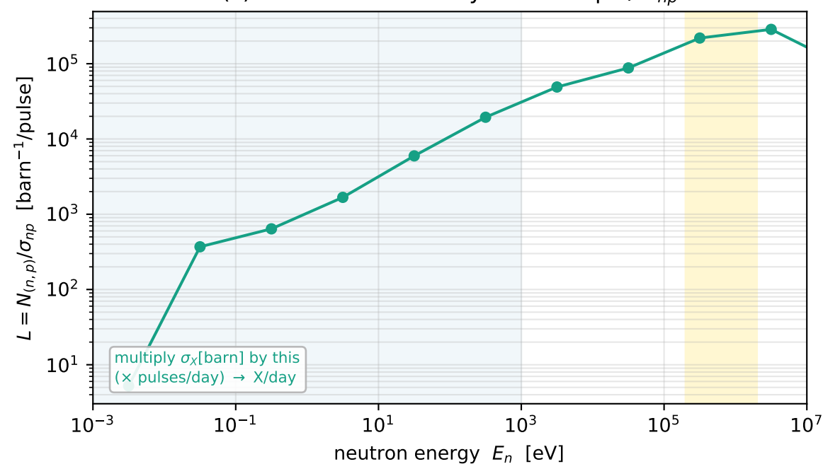
(c) effective luminosity = breakups / \sigma_{np}
