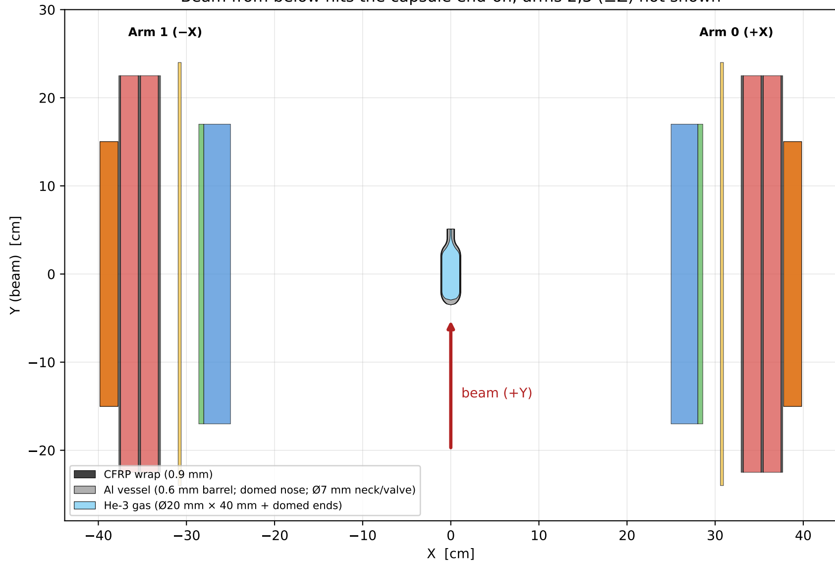
MX17 Geometry — Side View (XY plane) Beam from below hits the capsule end-on; arms 2,3 ( \pm Z ) not shown
