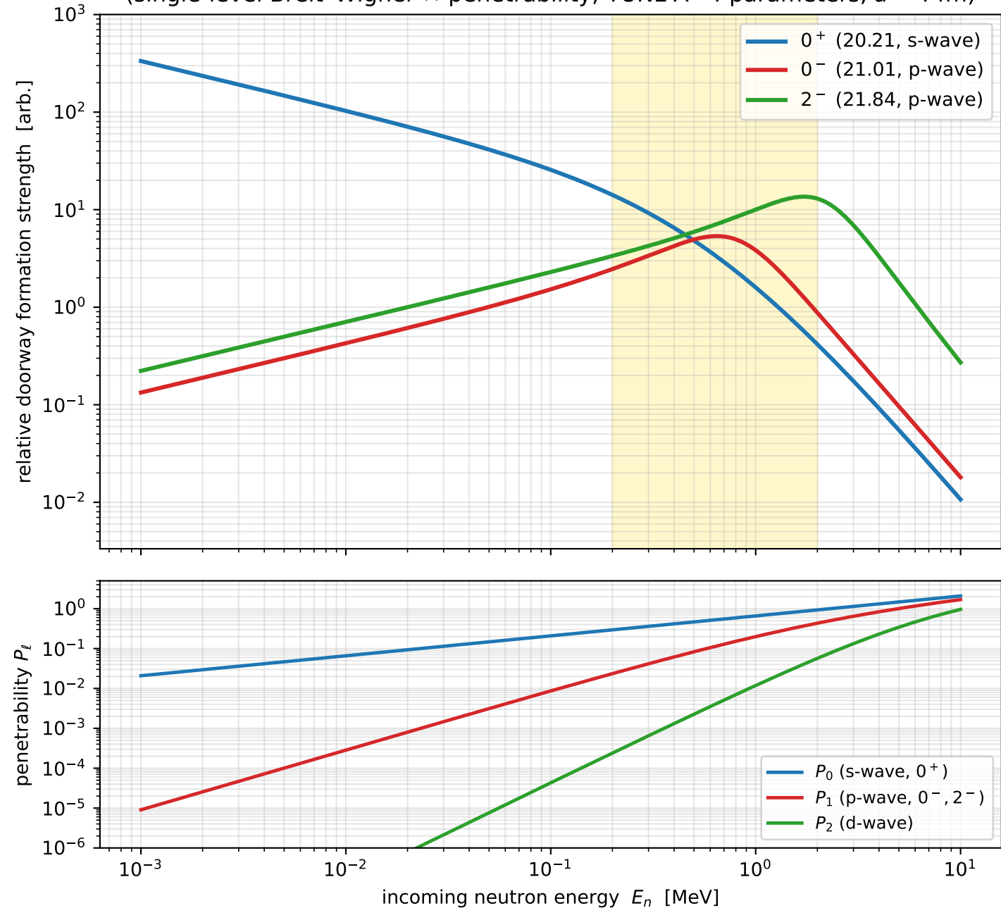
Forming {}^4\text{He}^* through the 0^+ vs 0^- doorway (single-level Breit-Wigner \times penetrability; TUNL A=4 parameters, a = 4 fm)
