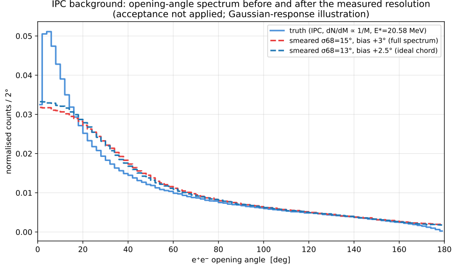
Figure 8: The IPC background spectrum before and after the measured resolution (same construction as the X17 dilution plot in Part I; the virtual-state mass is sampled from the generator’s dN/dM \propto 1/M ). The one structure IPC has — the small-angle pile-up from low-mass pairs — is flattened, and everything above \sim 60^\circ is essentially invariant : a smooth continuum smeared by 15^\circ is the same smooth continuum. The resolution damages only the signal.
