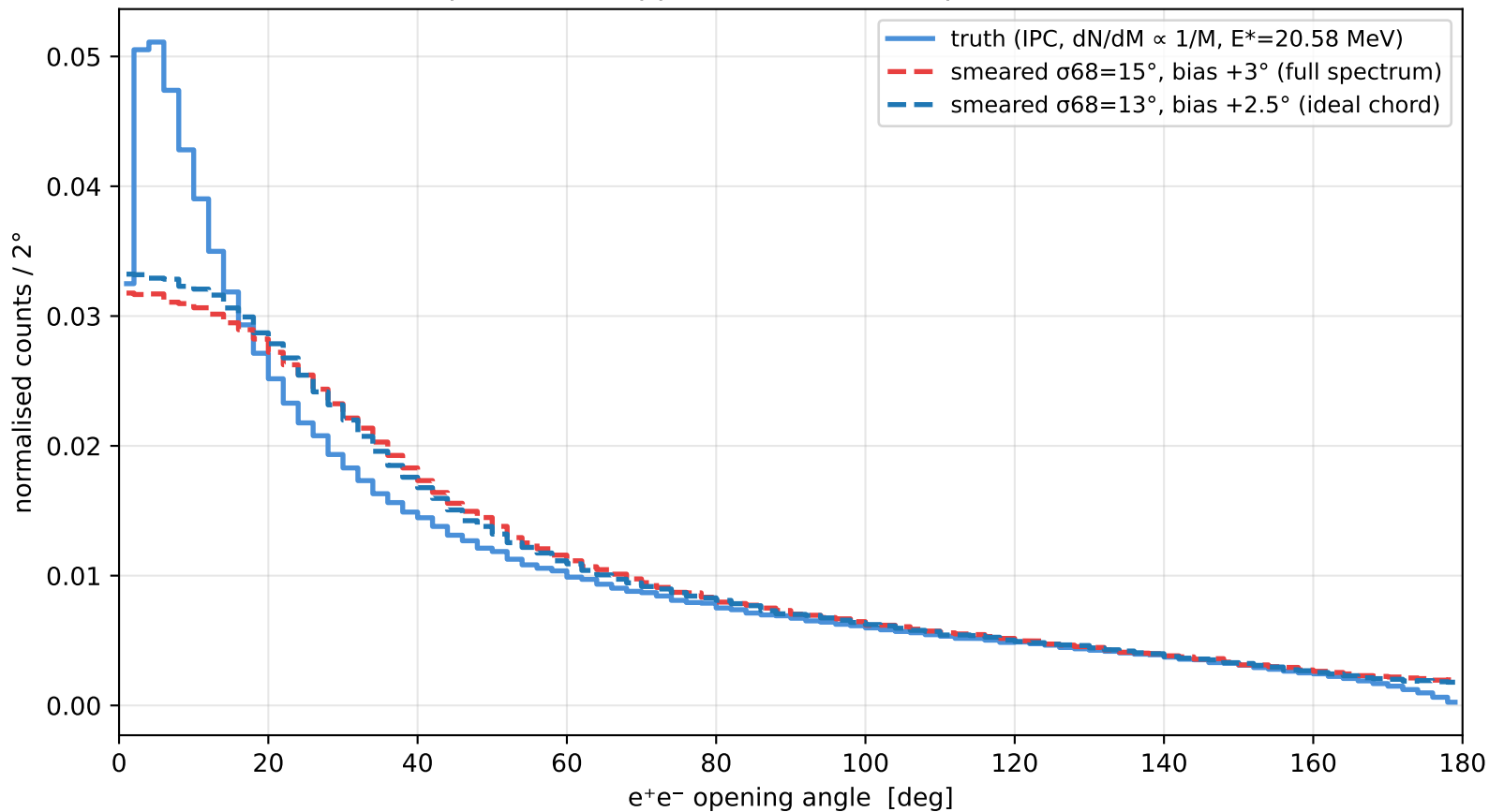
IPC background: opening-angle spectrum before and after the measured resolution (acceptance not applied; Gaussian-response illustration)
