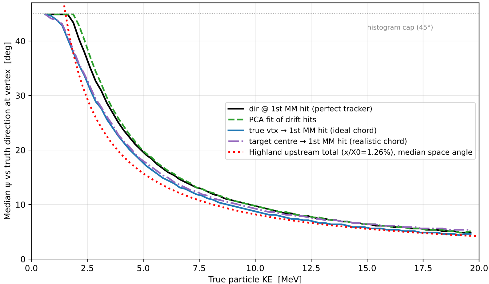
Per-particle direction error vs KE — pairs_v2 (10M events, STEP capsule) all estimators converge to the upstream-MS floor
