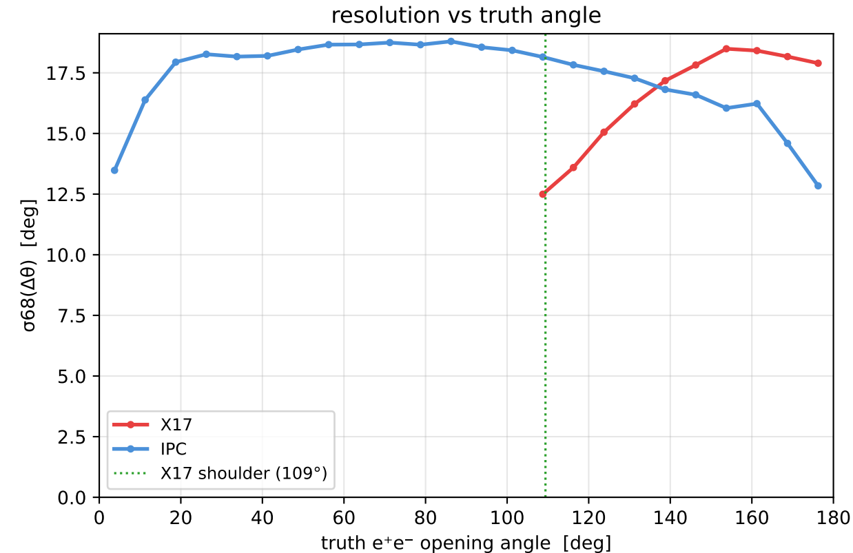
Opening-angle response vs truth angle, per species — per-leg P(\psi|KE) smearing, target-centre chord (X17 sharpest at its shoulder: symmetric pairs; boundary effects drive the bias at 0^\circ/180^\circ )
