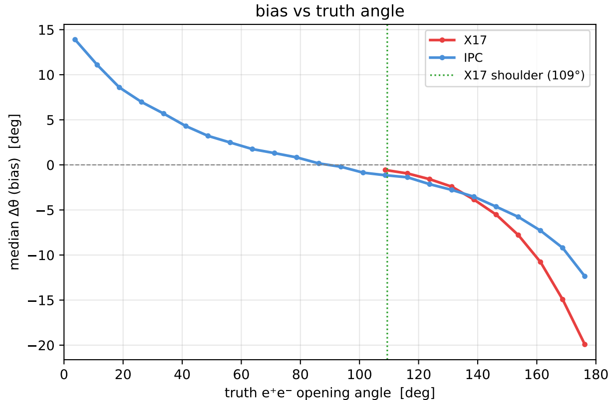
Opening-angle response vs truth angle, per species — per-leg P(\psi|KE) smearing, target-centre chord (X17 sharpest at its shoulder: symmetric pairs; boundary effects drive the bias at 0^\circ/180^\circ )
